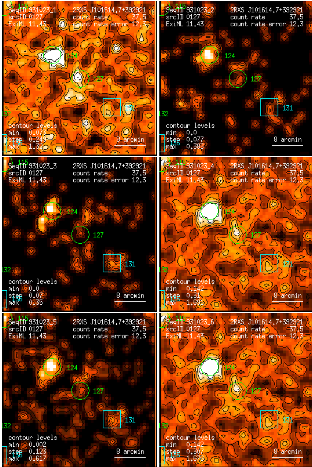
Figure 127: RASS 931023: detection 0127: band rate images, Gaussian filter: (1) PSPC channels 11 – 41, (2) 52 – 90, (3) 91 – 201, (4) 11 – 235, (5) 52 – 201, (6) 11 – 201. Broad band rates in counts/ks. Band rate contour levels in counts/ks/arcmin 2 .
