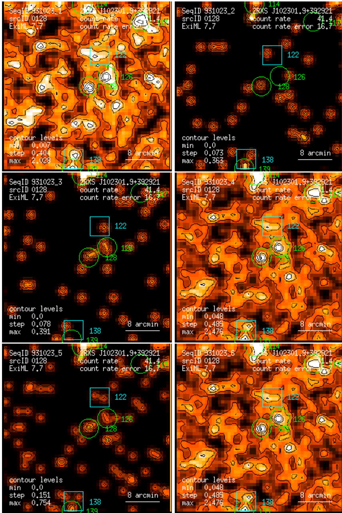
Figure 128: RASS 931023: detection 0128: band rate images, Gaussian filter: (1) PSPC channels 11 – 41, (2) 52 – 90, (3) 91 – 201, (4) 11 – 235, (5) 52 – 201, (6) 11 – 201. Broad band rates in counts/ks. Band rate contour levels in counts/ks/arcmin 2 .
