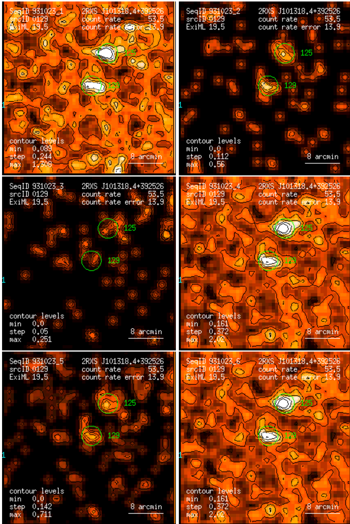
Figure 129: RASS 931023: detection 0129: band rate images, Gaussian filter: (1) PSPC channels 11 – 41, (2) 52 – 90, (3) 91 – 201, (4) 11 – 235, (5) 52 – 201, (6) 11 – 201. Broad band rates in counts/ks. Band rate contour levels in counts/ks/arcmin 2 .
