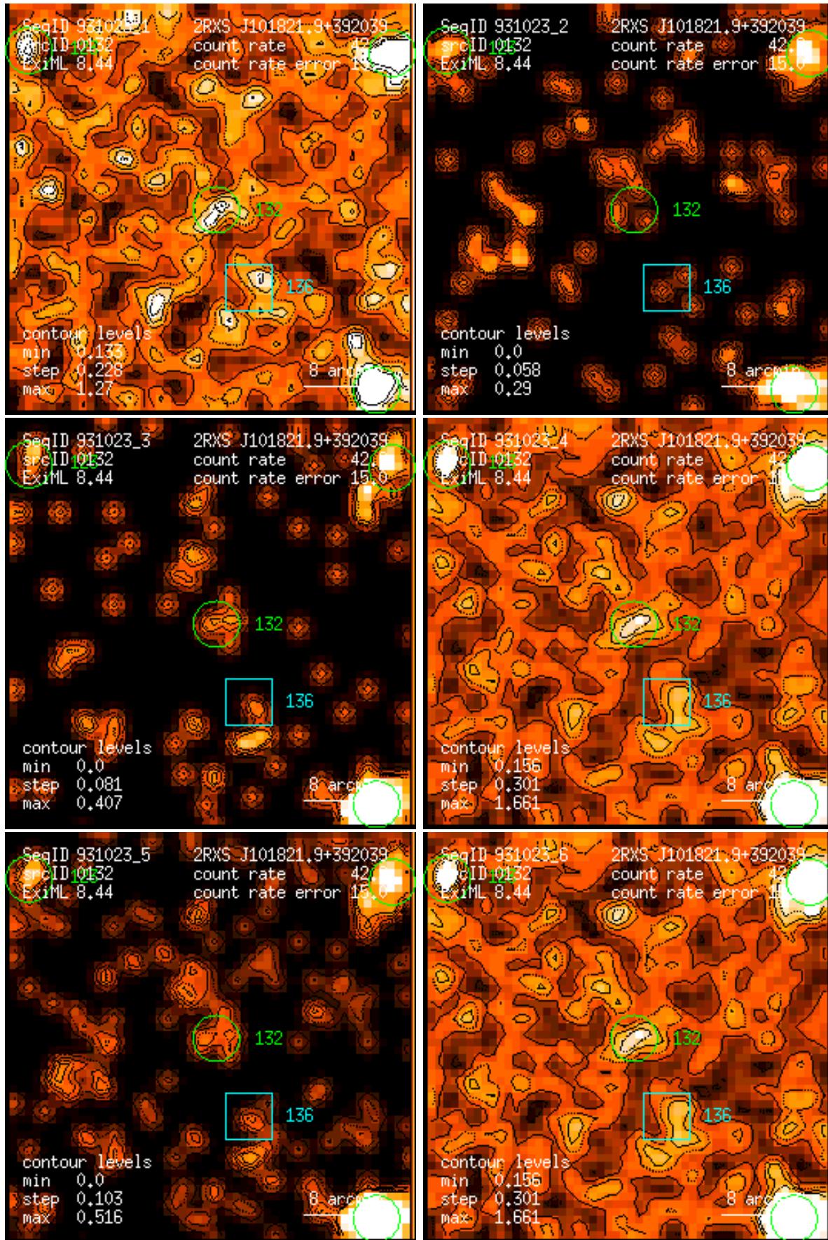
Figure 132: RASS 931023: detection 0132: band rate images, Gaussian filter: (1) PSPC channels 11 – 41, (2) 52 – 90, (3) 91 – 201, (4) 11 – 235, (5) 52 – 201, (6) 11 – 201. Broad band rates in counts/ks. Band rate contour levels in counts/ks/arcmin 2 .
