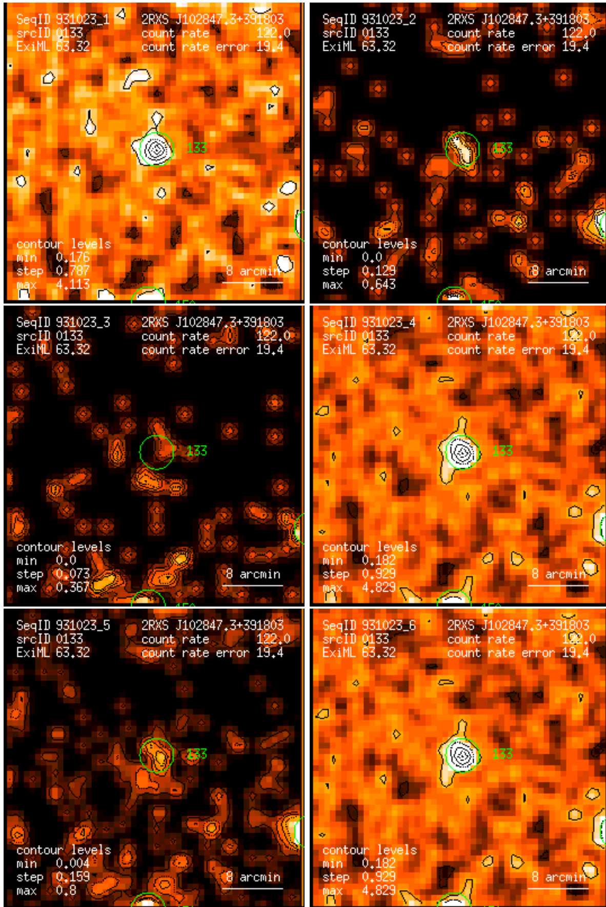
Figure 133: RASS 931023: detection 0133: band rate images, Gaussian filter: (1) PSPC channels 11 – 41, (2) 52 – 90, (3) 91 – 201, (4) 11 – 235, (5) 52 – 201, (6) 11 – 201. Broad band rates in counts/ks. Band rate contour levels in counts/ks/arcmin 2 .
