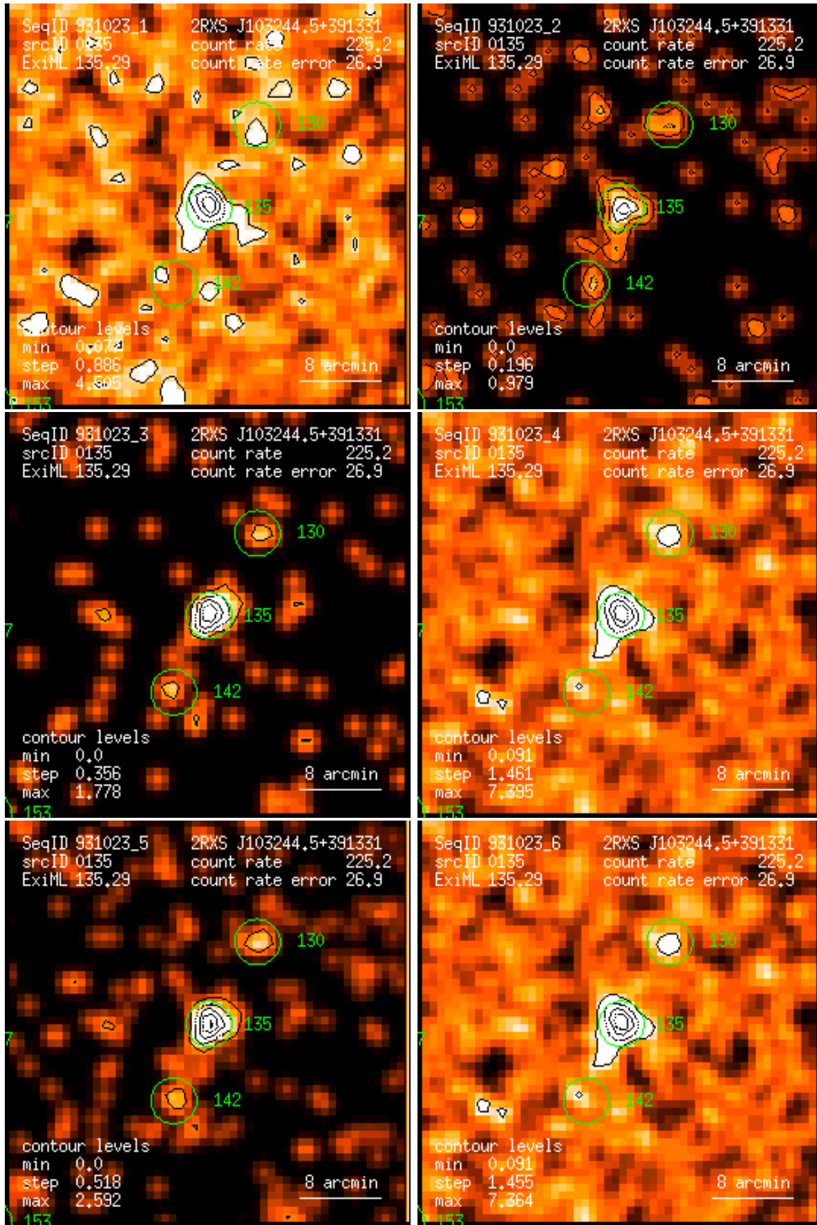
Figure 135: RASS 931023: detection 0135: band rate images, Gaussian filter: (1) PSPC channels 11 – 41, (2) 52 – 90, (3) 91 – 201, (4) 11 – 235, (5) 52 – 201, (6) 11 – 201. Broad band rates in counts/ks. Band rate contour levels in counts/ks/arcmin 2 .
