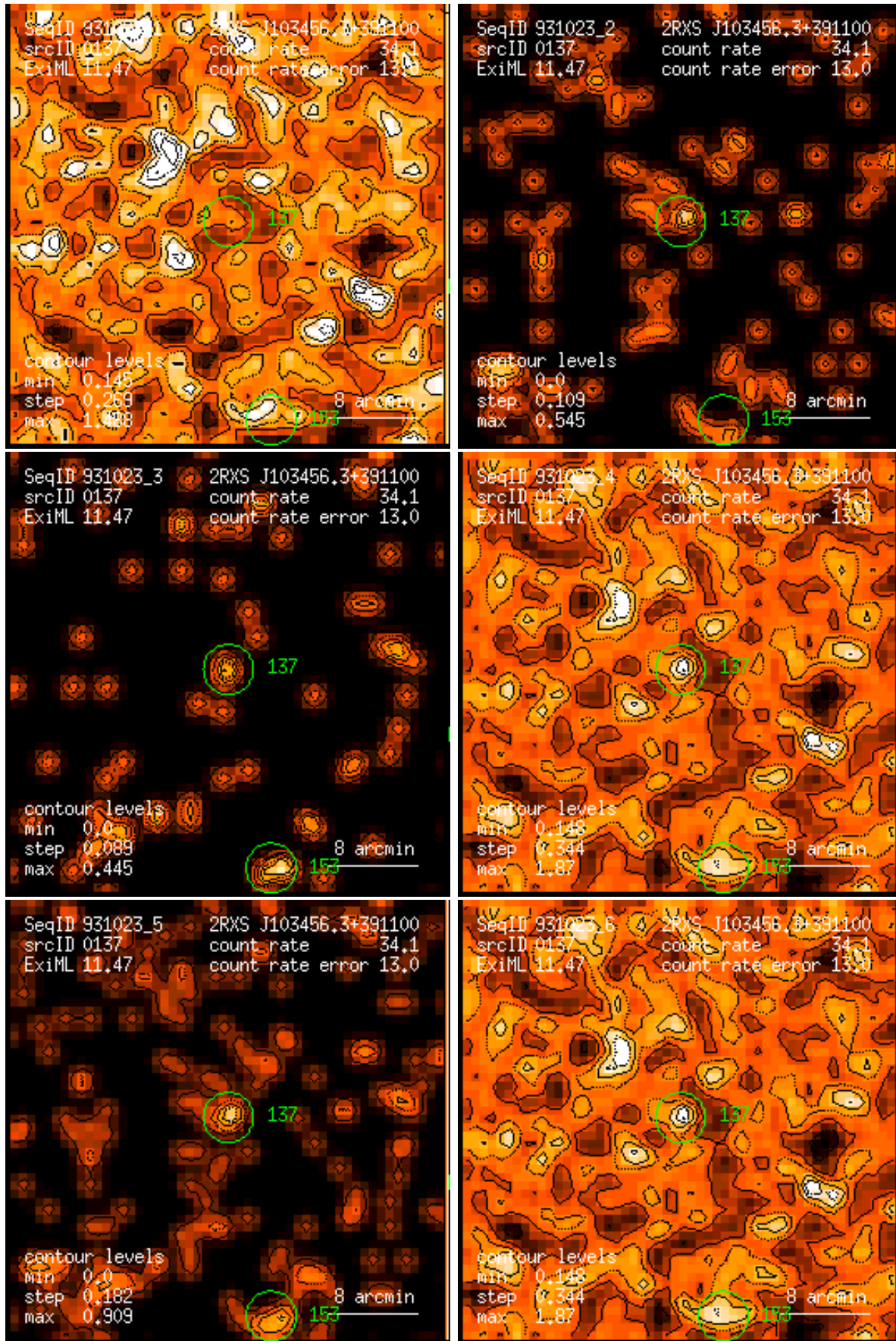
Figure 137: RASS 931023: detection 0137: band rate images, Gaussian filter: (1) PSPC channels 11 – 41, (2) 52 – 90, (3) 91 – 201, (4) 11 – 235, (5) 52 – 201, (6) 11 – 201. Broad band rates in counts/ks. Band rate contour levels in counts/ks/arcmin 2 .
