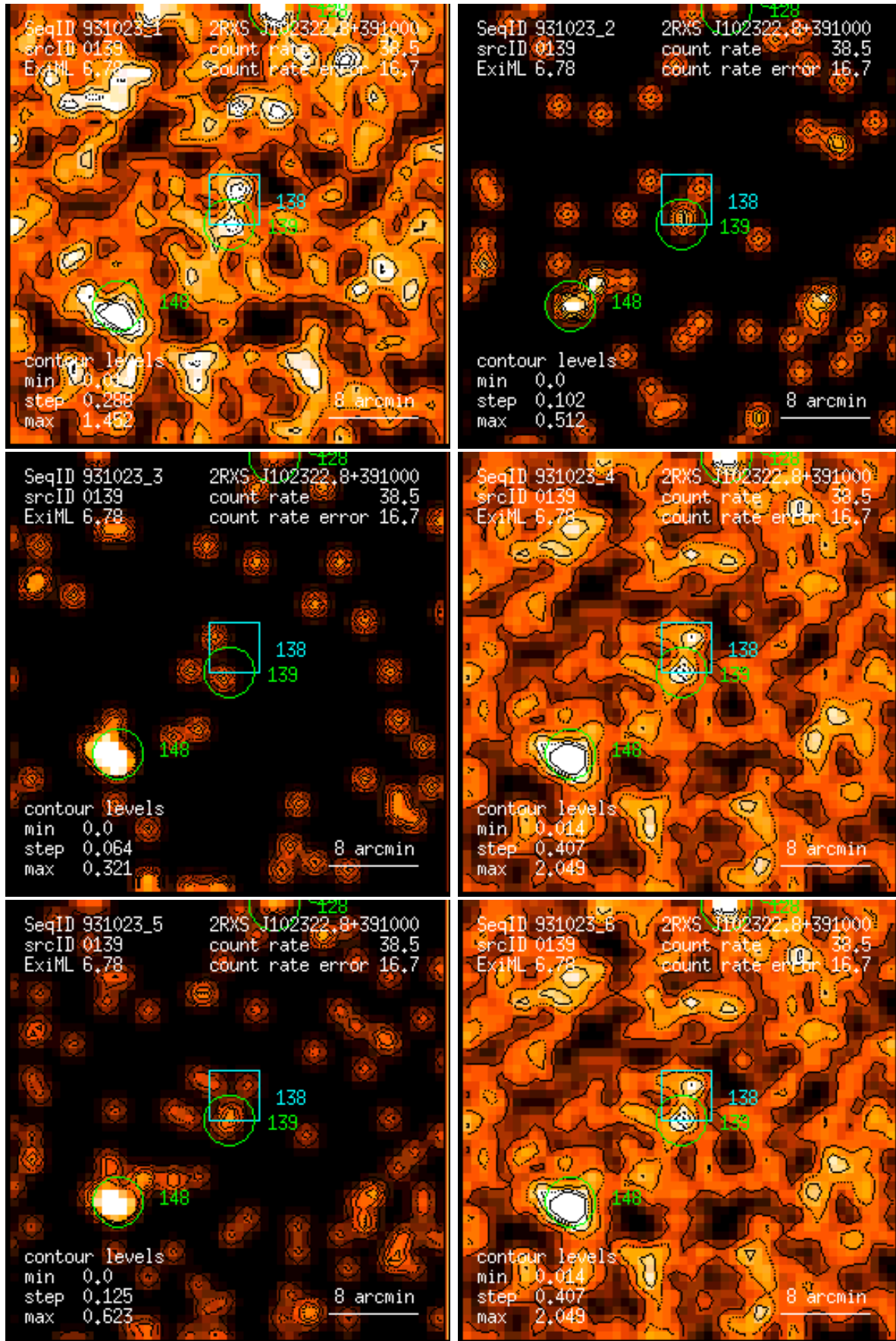
Figure 139: RASS 931023: detection 0139: band rate images, Gaussian filter: (1) PSPC channels 11 – 41, (2) 52 – 90, (3) 91 – 201, (4) 11 – 235, (5) 52 – 201, (6) 11 – 201. Broad band rates in counts/ks. Band rate contour levels in counts/ks/arcmin 2 .
