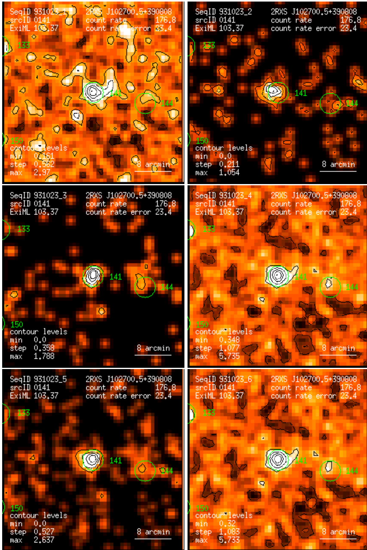
Figure 141: RASS 931023: detection 0141: band rate images, Gaussian filter: (1) PSPC channels 11 – 41, (2) 52 – 90, (3) 91 – 201, (4) 11 – 235, (5) 52 – 201, (6) 11 – 201. Broad band rates in counts/ks. Band rate contour levels in counts/ks/arcmin 2 .
