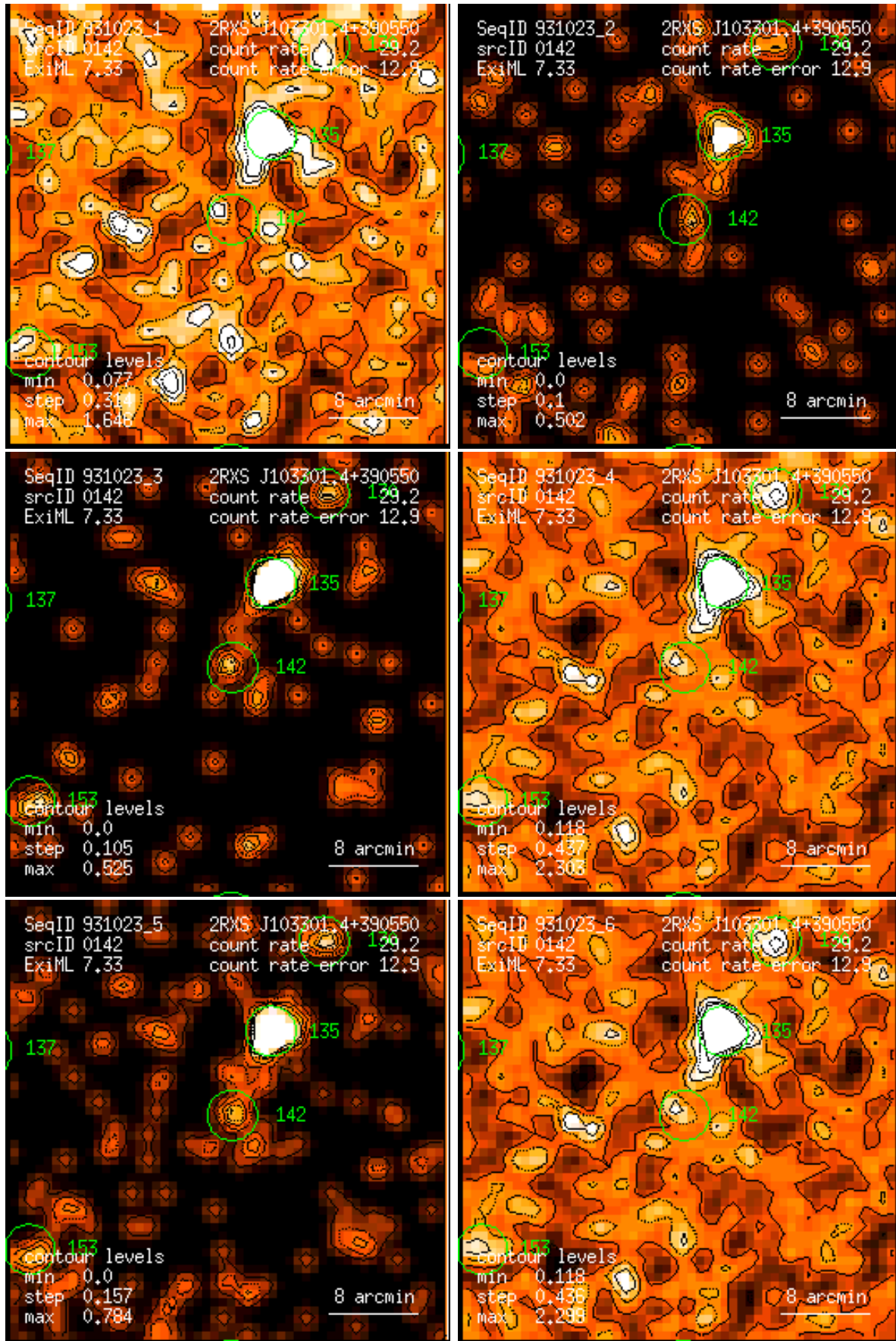
Figure 142: RASS 931023: detection 0142: band rate images, Gaussian filter: (1) PSPC channels 11 – 41, (2) 52 – 90, (3) 91 – 201, (4) 11 – 235, (5) 52 – 201, (6) 11 – 201. Broad band rates in counts/ks. Band rate contour levels in counts/ks/arcmin 2 .
