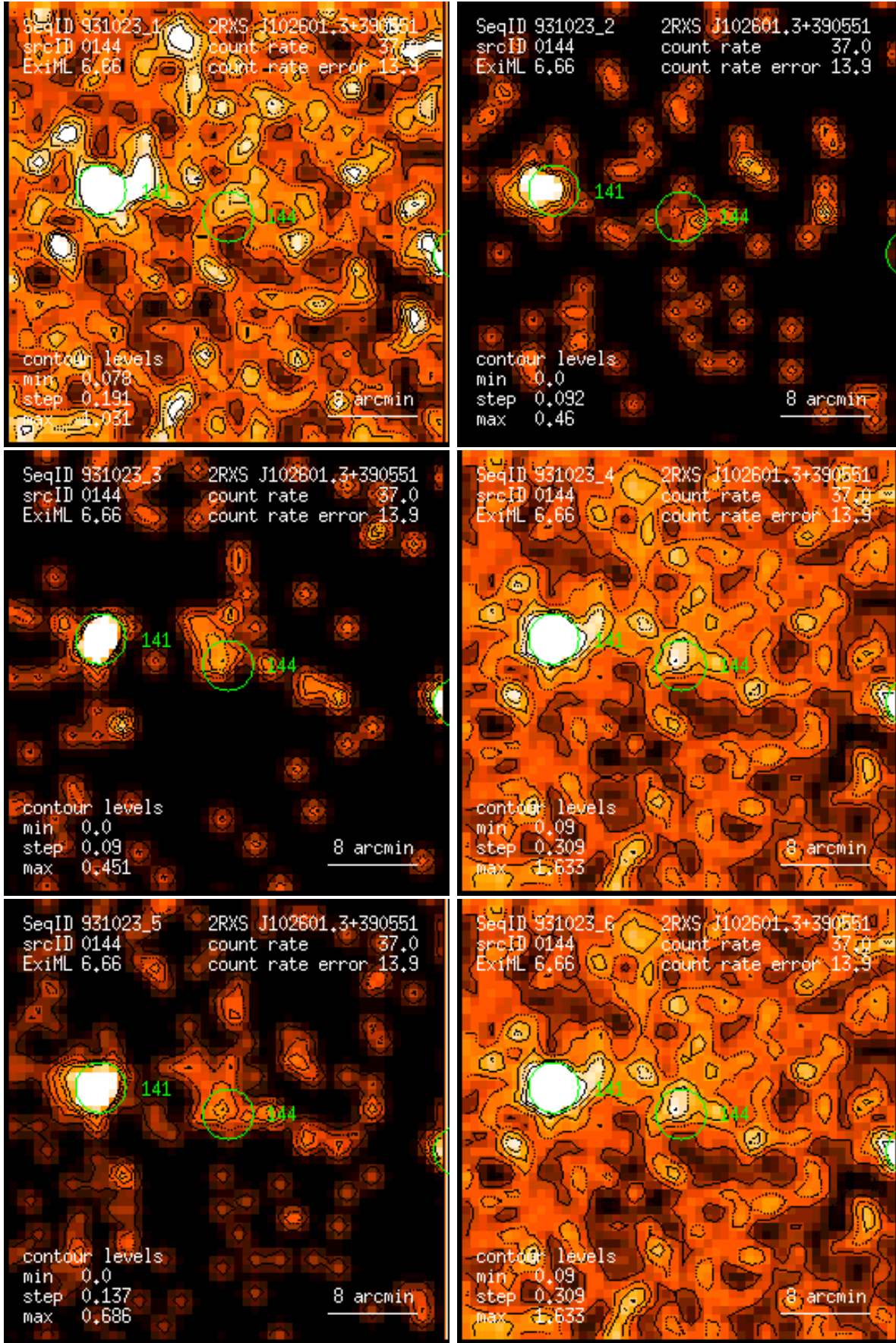
Figure 144: RASS 931023: detection 0144: band rate images, Gaussian filter: (1) PSPC channels 11 – 41, (2) 52 – 90, (3) 91 – 201, (4) 11 – 235, (5) 52 – 201, (6) 11 – 201. Broad band rates in counts/ks. Band rate contour levels in counts/ks/arcmin 2 .
