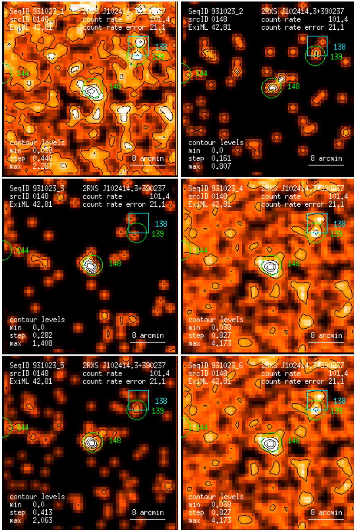
Figure 148: RASS 931023: detection 0148: band rate images, Gaussian filter: (1) PSPC channels 11 – 41, (2) 52 – 90, (3) 91 – 201, (4) 11 – 235, (5) 52 – 201, (6) 11 – 201. Broad band rates in counts/ks. Band rate contour levels in counts/ks/arcmin 2 .
