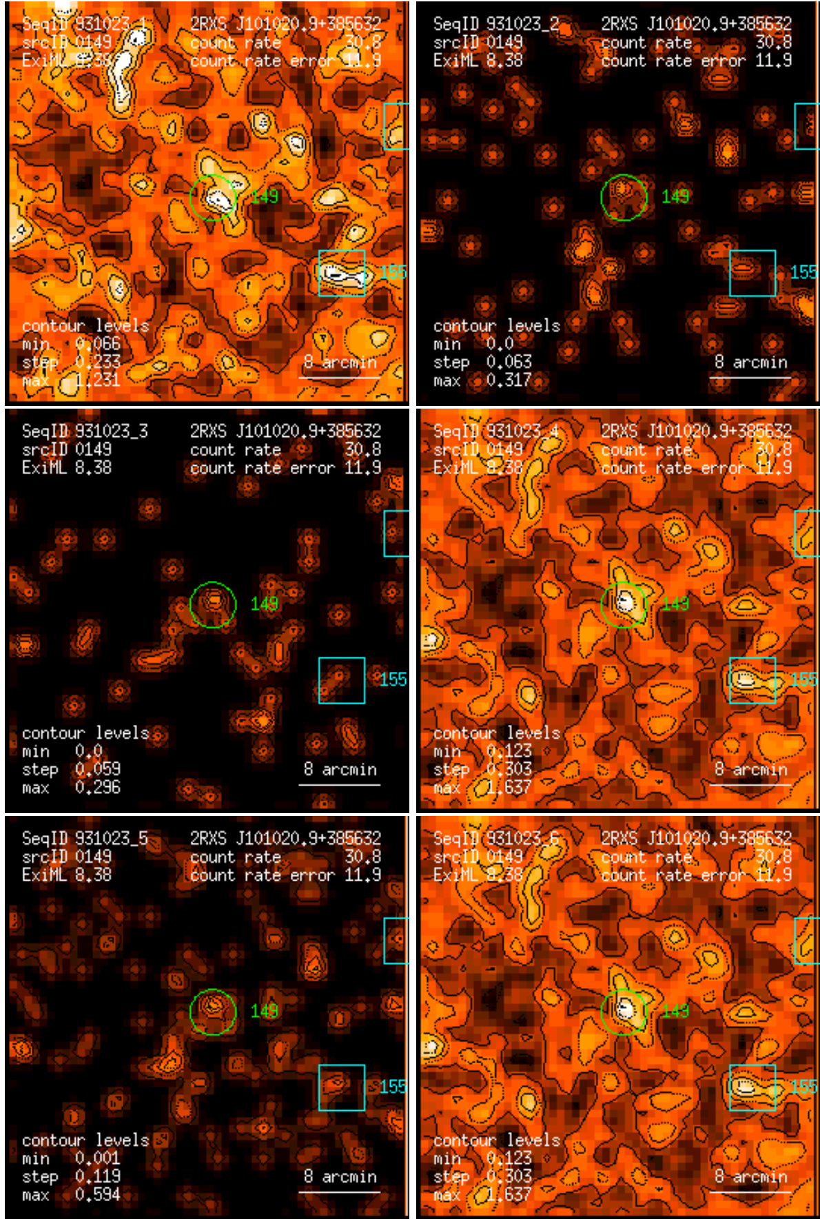
Figure 149: RASS 931023: detection 0149: band rate images, Gaussian filter: (1) PSPC channels 11 – 41, (2) 52 – 90, (3) 91 – 201, (4) 11 – 235, (5) 52 – 201, (6) 11 – 201. Broad band rates in counts/ks. Band rate contour levels in counts/ks/arcmin 2 .
