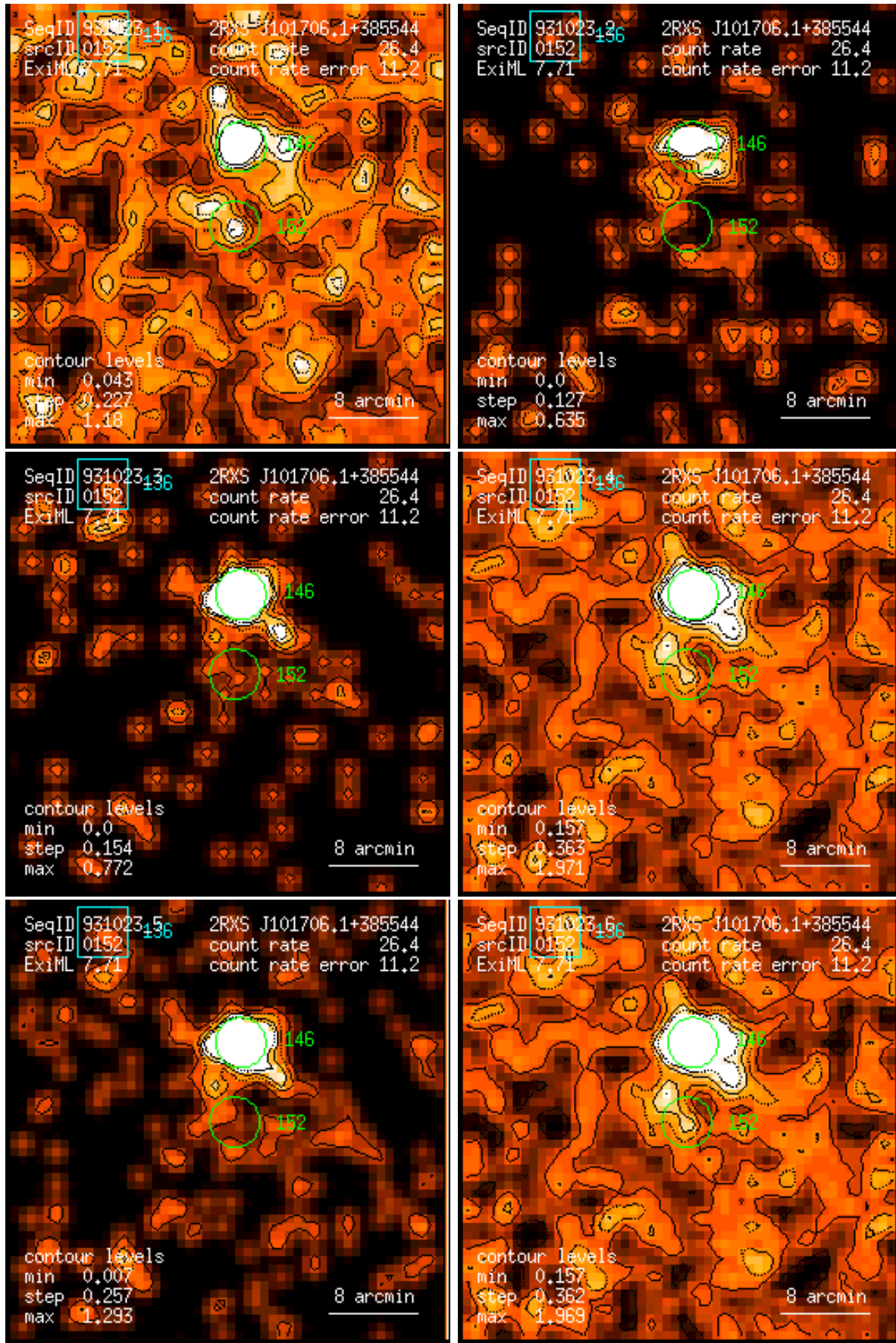
Figure 152: RASS 931023: detection 0152: band rate images, Gaussian filter: (1) PSPC channels 11 – 41, (2) 52 – 90, (3) 91 – 201, (4) 11 – 235, (5) 52 – 201, (6) 11 – 201. Broad band rates in counts/ks. Band rate contour levels in counts/ks/arcmin 2 .
