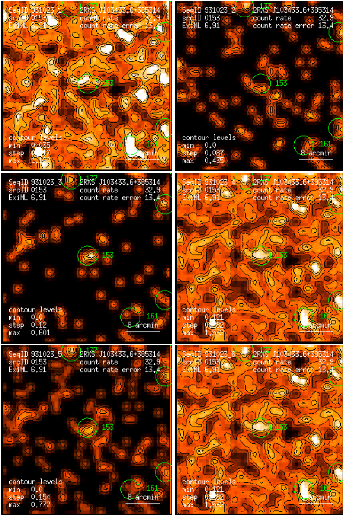
Figure 153: RASS 931023: detection 0153: band rate images, Gaussian filter: (1) PSPC channels 11 – 41, (2) 52 – 90, (3) 91 – 201, (4) 11 – 235, (5) 52 – 201, (6) 11 – 201. Broad band rates in counts/ks. Band rate contour levels in counts/ks/arcmin 2 .
