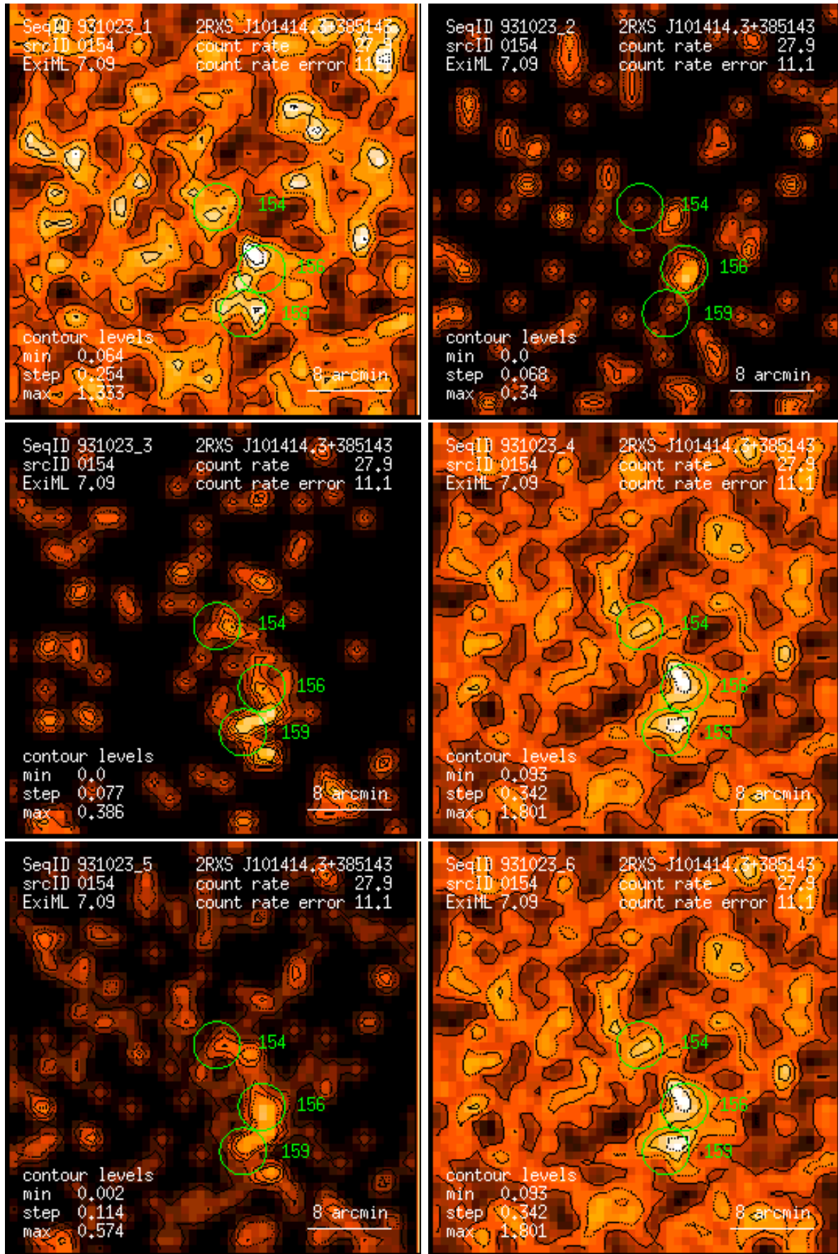
Figure 154: RASS 931023: detection 0154: band rate images, Gaussian filter: (1) PSPC channels 11 – 41, (2) 52 – 90, (3) 91 – 201, (4) 11 – 235, (5) 52 – 201, (6) 11 – 201. Broad band rates in counts/ks. Band rate contour levels in counts/ks/arcmin 2 .
