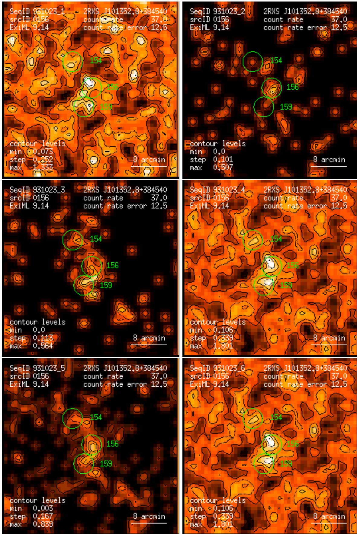
Figure 156: RASS 931023: detection 0156: band rate images, Gaussian filter: (1) PSPC channels 11 – 41, (2) 52 – 90, (3) 91 – 201, (4) 11 – 235, (5) 52 – 201, (6) 11 – 201. Broad band rates in counts/ks. Band rate contour levels in counts/ks/arcmin 2 .
