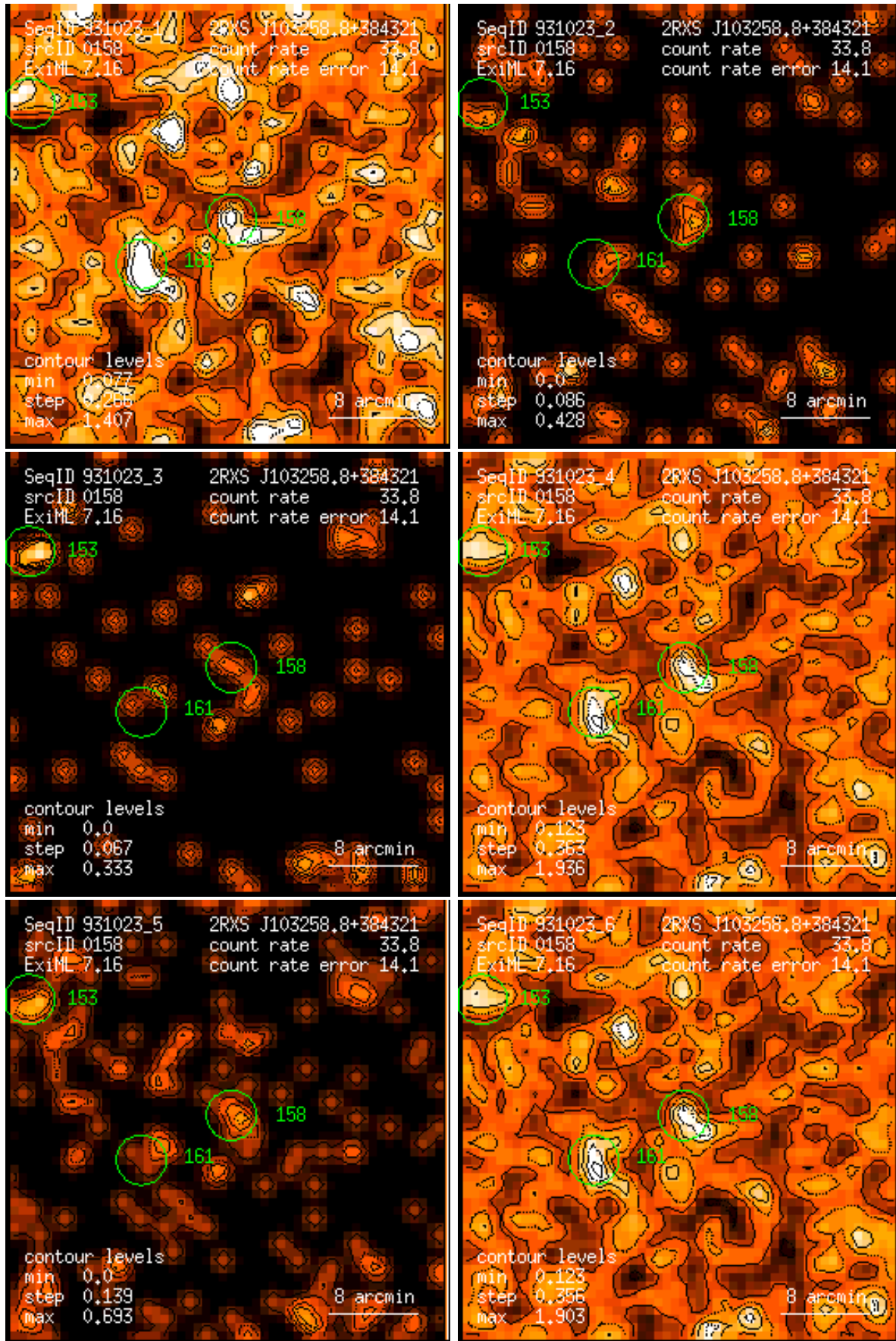
Figure 158: RASS 931023: detection 0158: band rate images, Gaussian filter: (1) PSPC channels 11 – 41, (2) 52 – 90, (3) 91 – 201, (4) 11 – 235, (5) 52 – 201, (6) 11 – 201. Broad band rates in counts/ks. Band rate contour levels in counts/ks/arcmin 2 .
