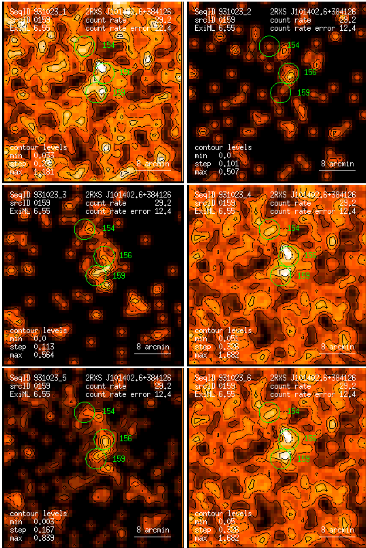
Figure 159: RASS 931023: detection 0159: band rate images, Gaussian filter: (1) PSPC channels 11 – 41, (2) 52 – 90, (3) 91 – 201, (4) 11 – 235, (5) 52 – 201, (6) 11 – 201. Broad band rates in counts/ks. Band rate contour levels in counts/ks/arcmin 2 .
