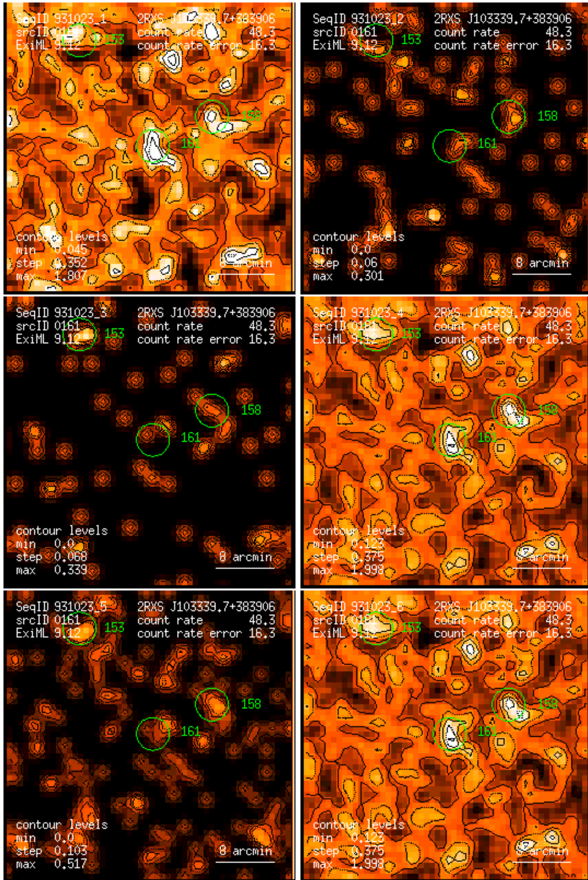
Figure 161: RASS 931023: detection 0161: band rate images, Gaussian filter: (1) PSPC channels 11 – 41, (2) 52 – 90, (3) 91 – 201, (4) 11 – 235, (5) 52 – 201, (6) 11 – 201. Broad band rates in counts/ks. Band rate contour levels in counts/ks/arcmin 2 .
