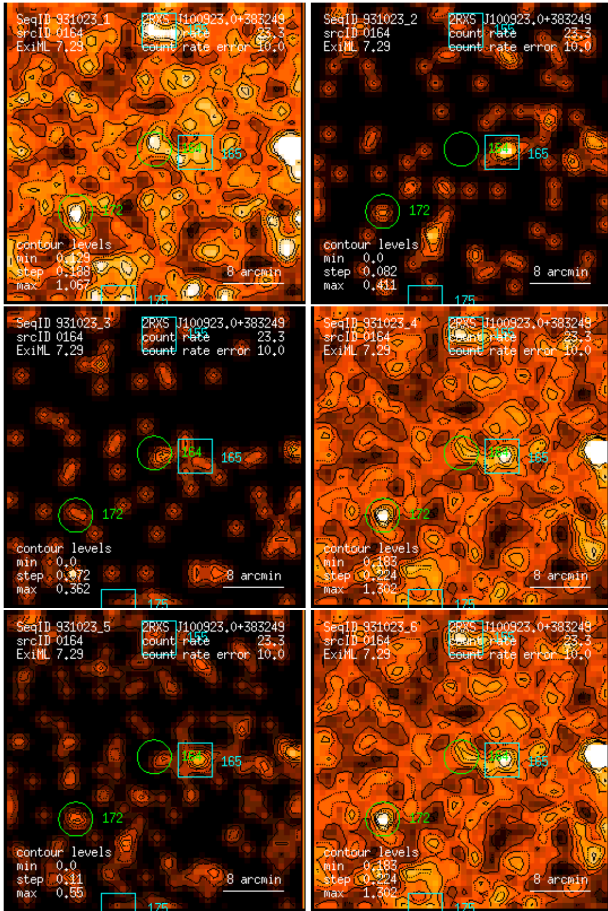
Figure 164: RASS 931023: detection 0164: band rate images, Gaussian filter: (1) PSPC channels 11 – 41, (2) 52 – 90, (3) 91 – 201, (4) 11 – 235, (5) 52 – 201, (6) 11 – 201. Broad band rates in counts/ks. Band rate contour levels in counts/ks/arcmin 2 .
