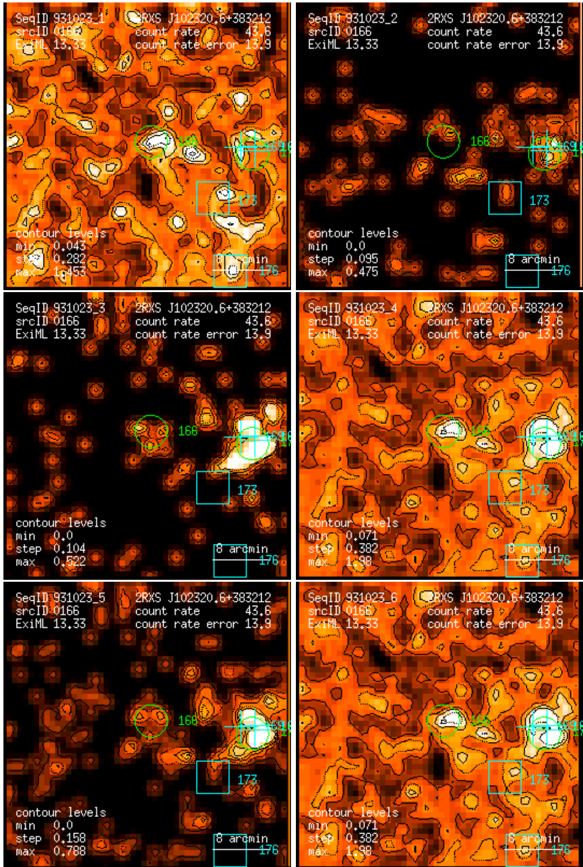
Figure 166: RASS 931023: detection 0166: band rate images, Gaussian filter: (1) PSPC channels 11 – 41, (2) 52 – 90, (3) 91 – 201, (4) 11 – 235, (5) 52 – 201, (6) 11 – 201. Broad band rates in counts/ks. Band rate contour levels in counts/ks/arcmin 2 .
