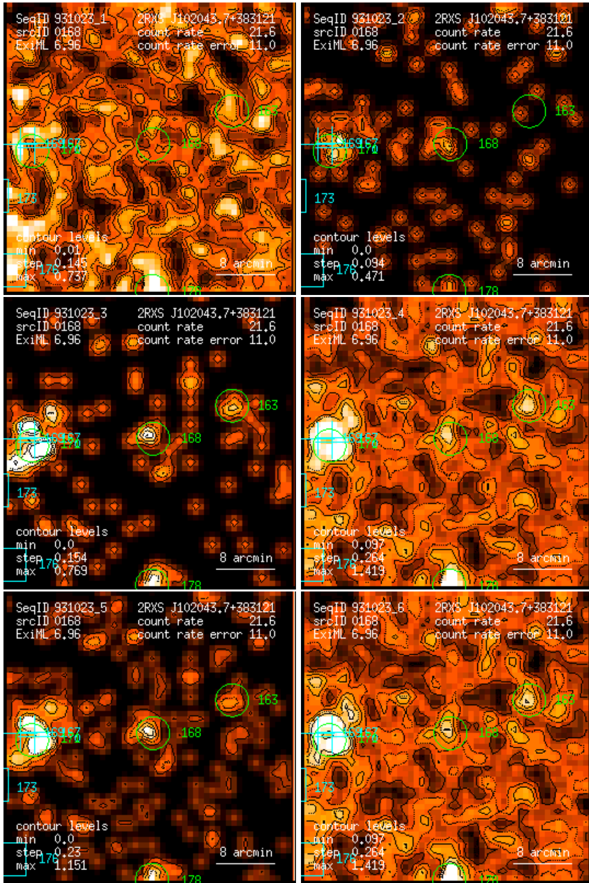
Figure 168: RASS 931023: detection 0168: band rate images, Gaussian filter: (1) PSPC channels 11 – 41, (2) 52 – 90, (3) 91 – 201, (4) 11 – 235, (5) 52 – 201, (6) 11 – 201. Broad band rates in counts/ks. Band rate contour levels in counts/ks/arcmin 2 .
