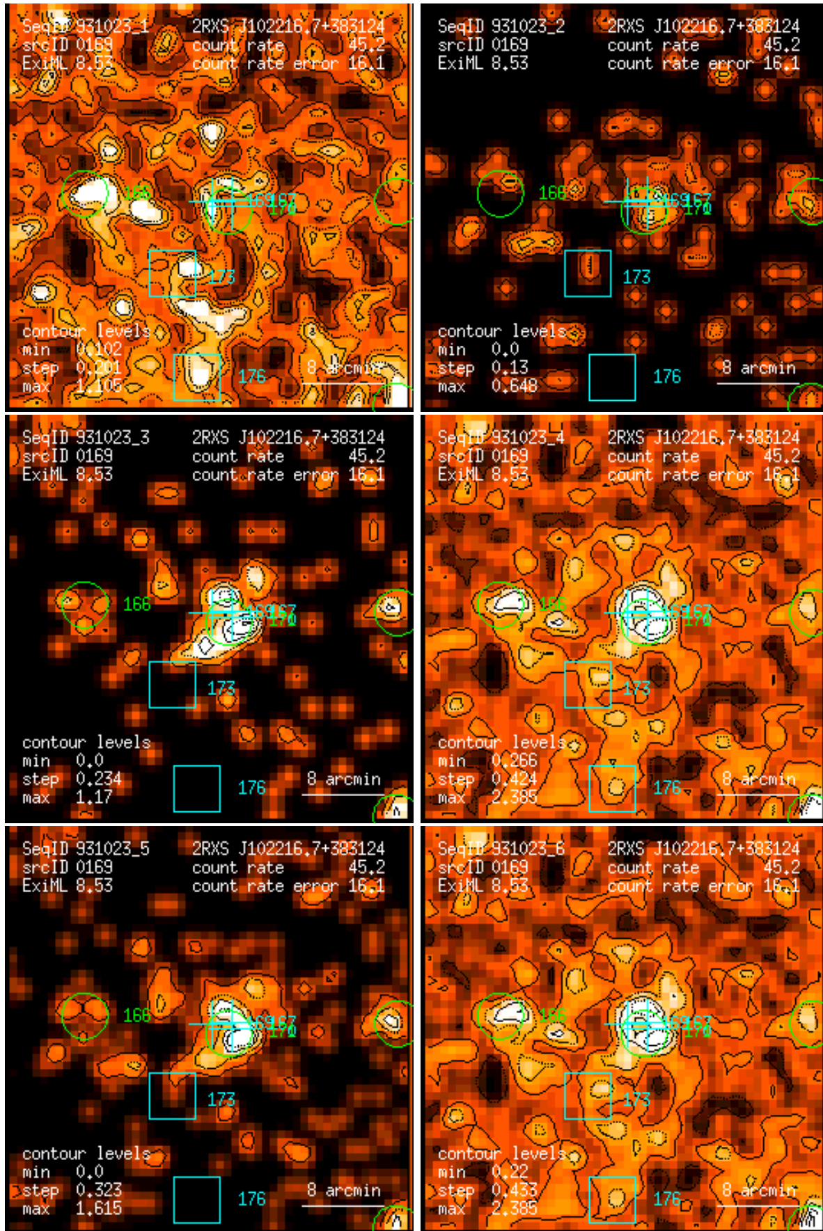
Figure 169: RASS 931023: detection 0169: band rate images, Gaussian filter: (1) PSPC channels 11 – 41, (2) 52 – 90, (3) 91 – 201, (4) 11 – 235, (5) 52 – 201, (6) 11 – 201. Broad band rates in counts/ks. Band rate contour levels in counts/ks/arcmin 2 .
