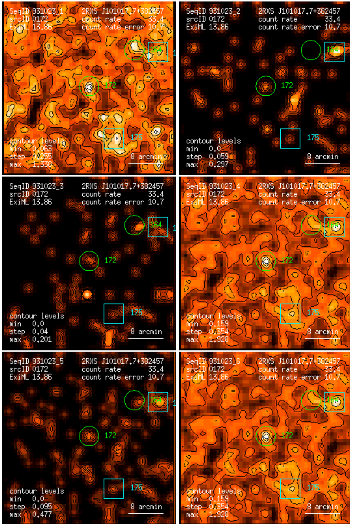
Figure 172: RASS 931023: detection 0172: band rate images, Gaussian filter: (1) PSPC channels 11 – 41, (2) 52 – 90, (3) 91 – 201, (4) 11 – 235, (5) 52 – 201, (6) 11 – 201. Broad band rates in counts/ks. Band rate contour levels in counts/ks/arcmin 2 .
