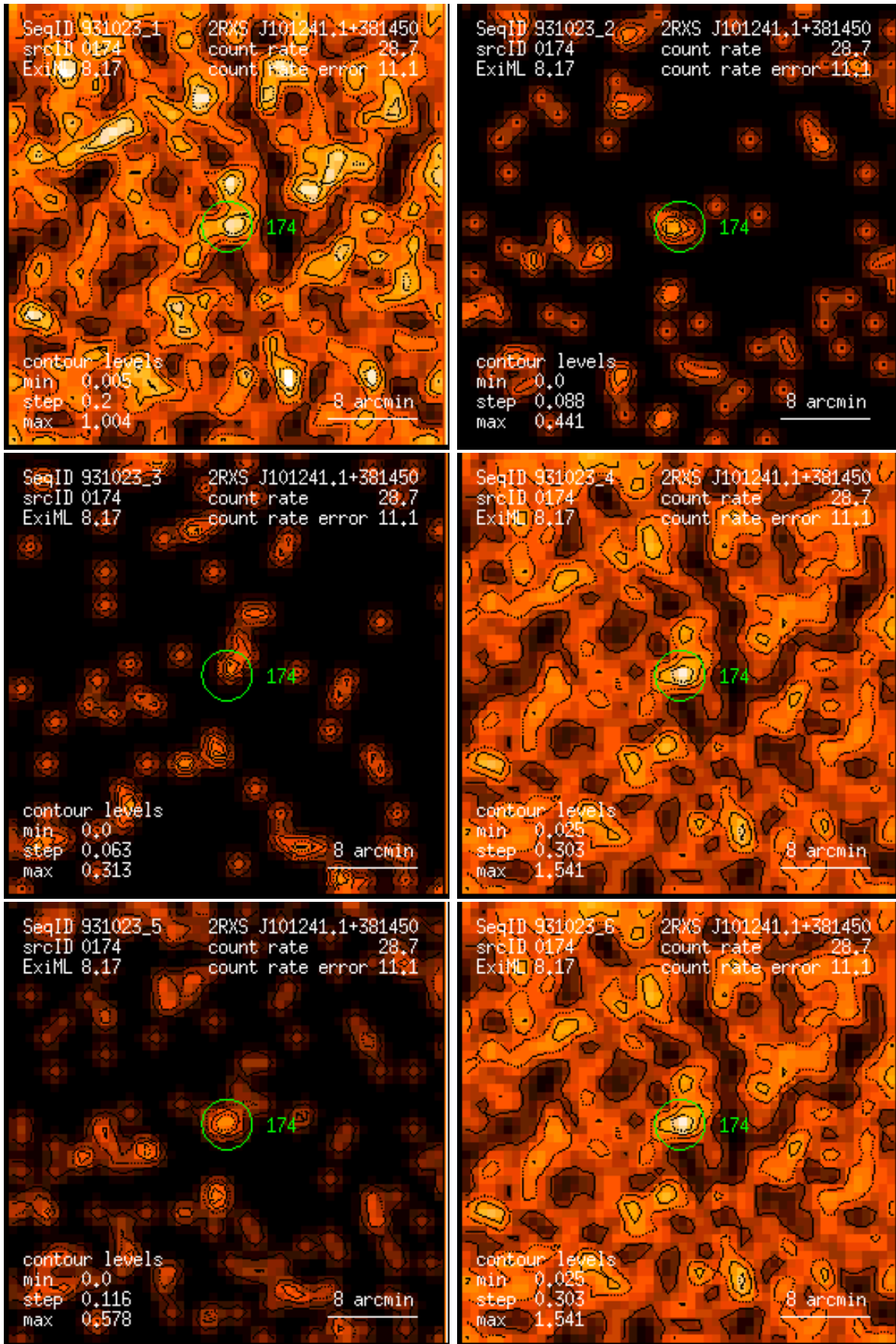
Figure 174: RASS 931023: detection 0174: band rate images, Gaussian filter: (1) PSPC channels 11 – 41, (2) 52 – 90, (3) 91 – 201, (4) 11 – 235, (5) 52 – 201, (6) 11 – 201. Broad band rates in counts/ks. Band rate contour levels in counts/ks/arcmin 2 .
