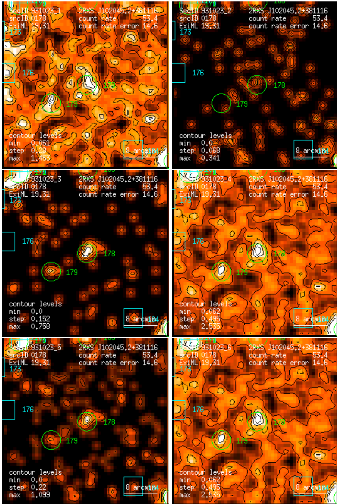
Figure 178: RASS 931023: detection 0178: band rate images, Gaussian filter: (1) PSPC channels 11 – 41, (2) 52 – 90, (3) 91 – 201, (4) 11 – 235, (5) 52 – 201, (6) 11 – 201. Broad band rates in counts/ks. Band rate contour levels in counts/ks/arcmin 2 .
