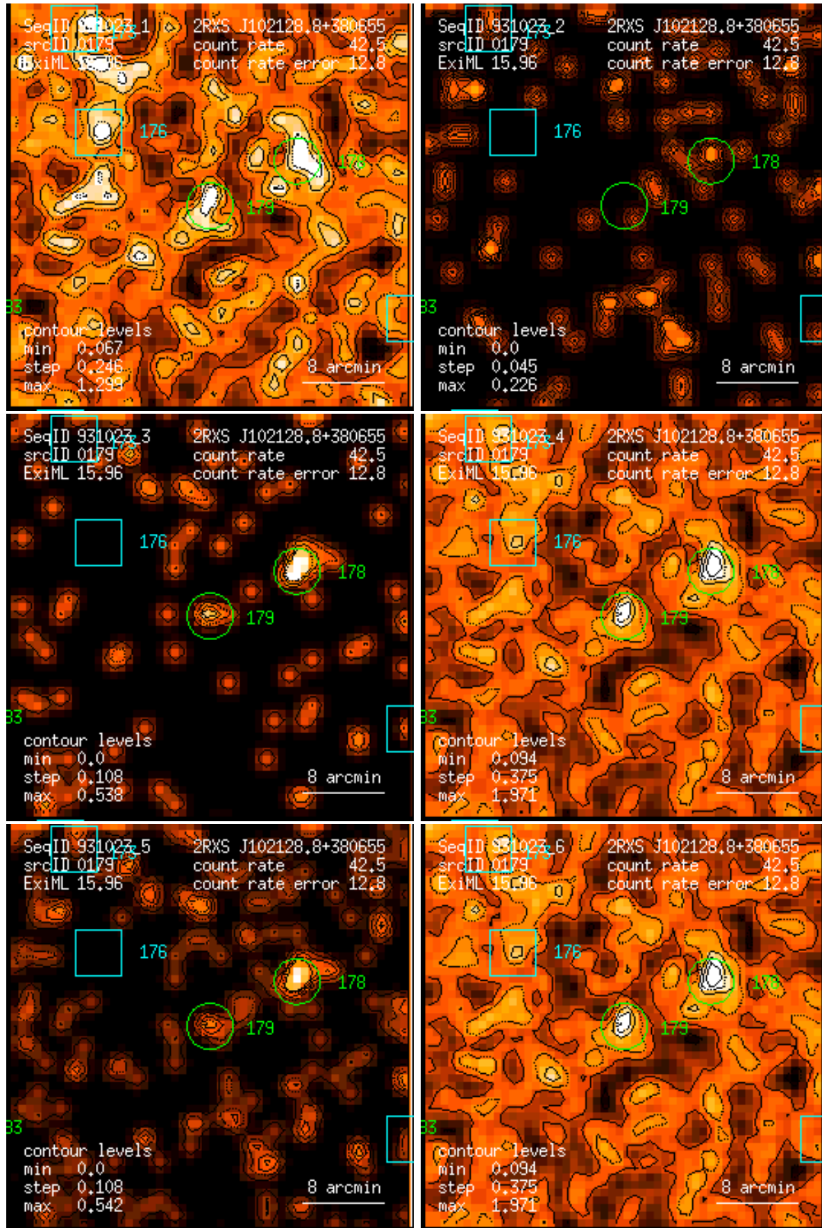
Figure 179: RASS 931023: detection 0179: band rate images, Gaussian filter: (1) PSPC channels 11 – 41, (2) 52 – 90, (3) 91 – 201, (4) 11 – 235, (5) 52 – 201, (6) 11 – 201. Broad band rates in counts/ks. Band rate contour levels in counts/ks/arcmin 2 .
