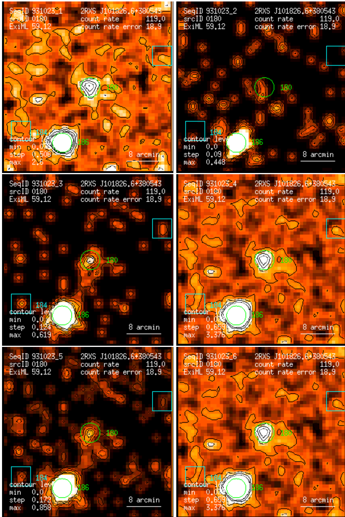
Figure 180: RASS 931023: detection 0180: band rate images, Gaussian filter: (1) PSPC channels 11 – 41, (2) 52 – 90, (3) 91 – 201, (4) 11 – 235, (5) 52 – 201, (6) 11 – 201. Broad band rates in counts/ks. Band rate contour levels in counts/ks/arcmin 2 .
