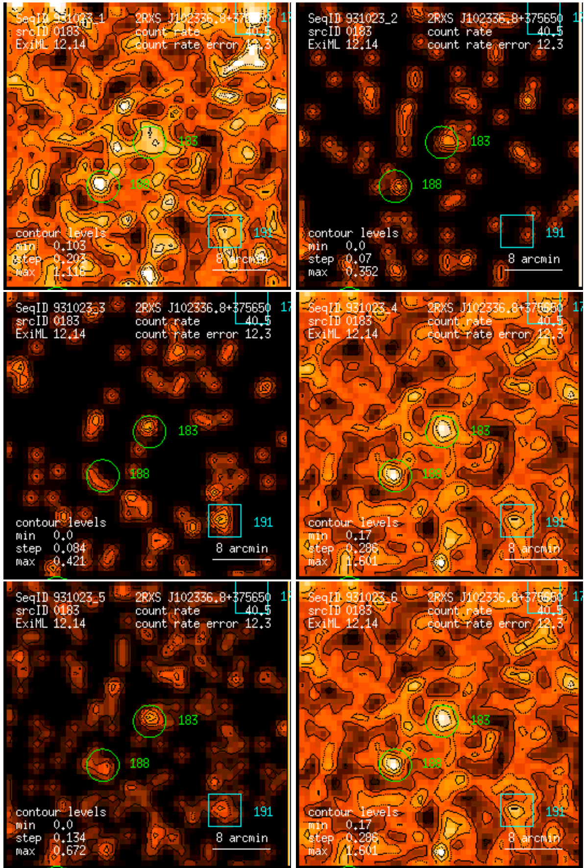
Figure 183: RASS 931023: detection 0183: band rate images, Gaussian filter: (1) PSPC channels 11 – 41, (2) 52 – 90, (3) 91 – 201, (4) 11 – 235, (5) 52 – 201, (6) 11 – 201. Broad band rates in counts/ks. Band rate contour levels in counts/ks/arcmin 2 .
