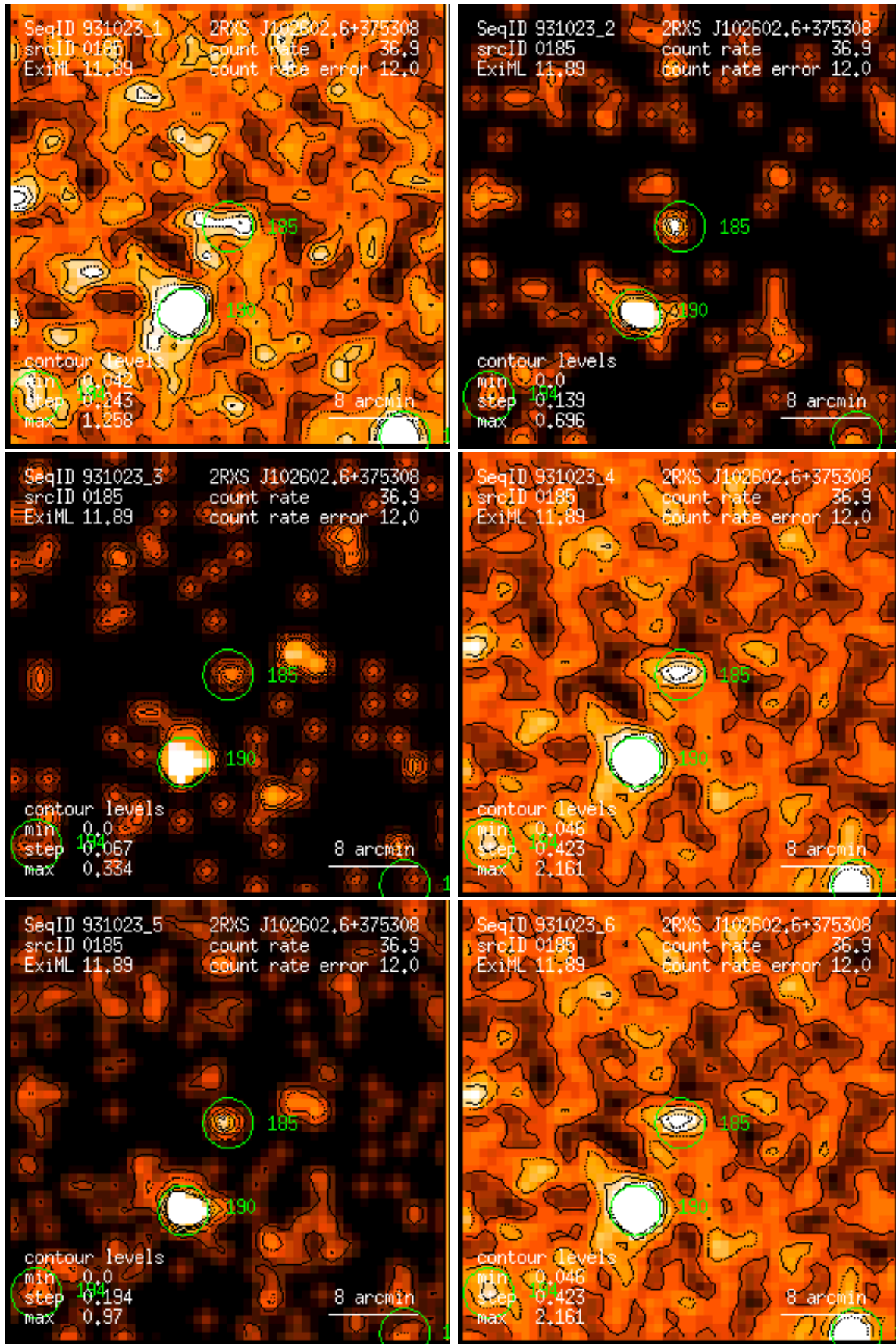
Figure 185: RASS 931023: detection 0185: band rate images, Gaussian filter: (1) PSPC channels 11 – 41, (2) 52 – 90, (3) 91 – 201, (4) 11 – 235, (5) 52 – 201, (6) 11 – 201. Broad band rates in counts/ks. Band rate contour levels in counts/ks/arcmin 2 .
