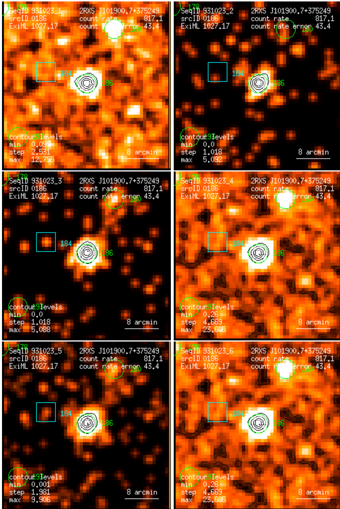
Figure 186: RASS 931023: detection 0186: band rate images, Gaussian filter: (1) PSPC channels 11 – 41, (2) 52 – 90, (3) 91 – 201, (4) 11 – 235, (5) 52 – 201, (6) 11 – 201. Broad band rates in counts/ks. Band rate contour levels in counts/ks/arcmin 2 .
