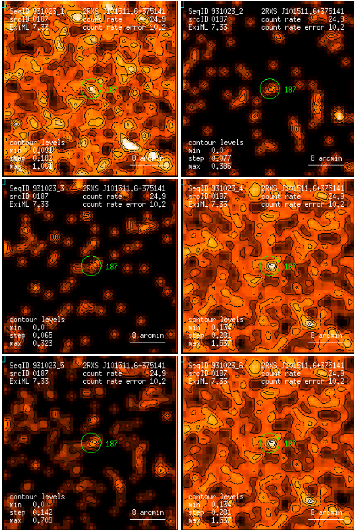
Figure 187: RASS 931023: detection 0187: band rate images, Gaussian filter: (1) PSPC channels 11 – 41, (2) 52 – 90, (3) 91 – 201, (4) 11 – 235, (5) 52 – 201, (6) 11 – 201. Broad band rates in counts/ks. Band rate contour levels in counts/ks/arcmin 2 .
