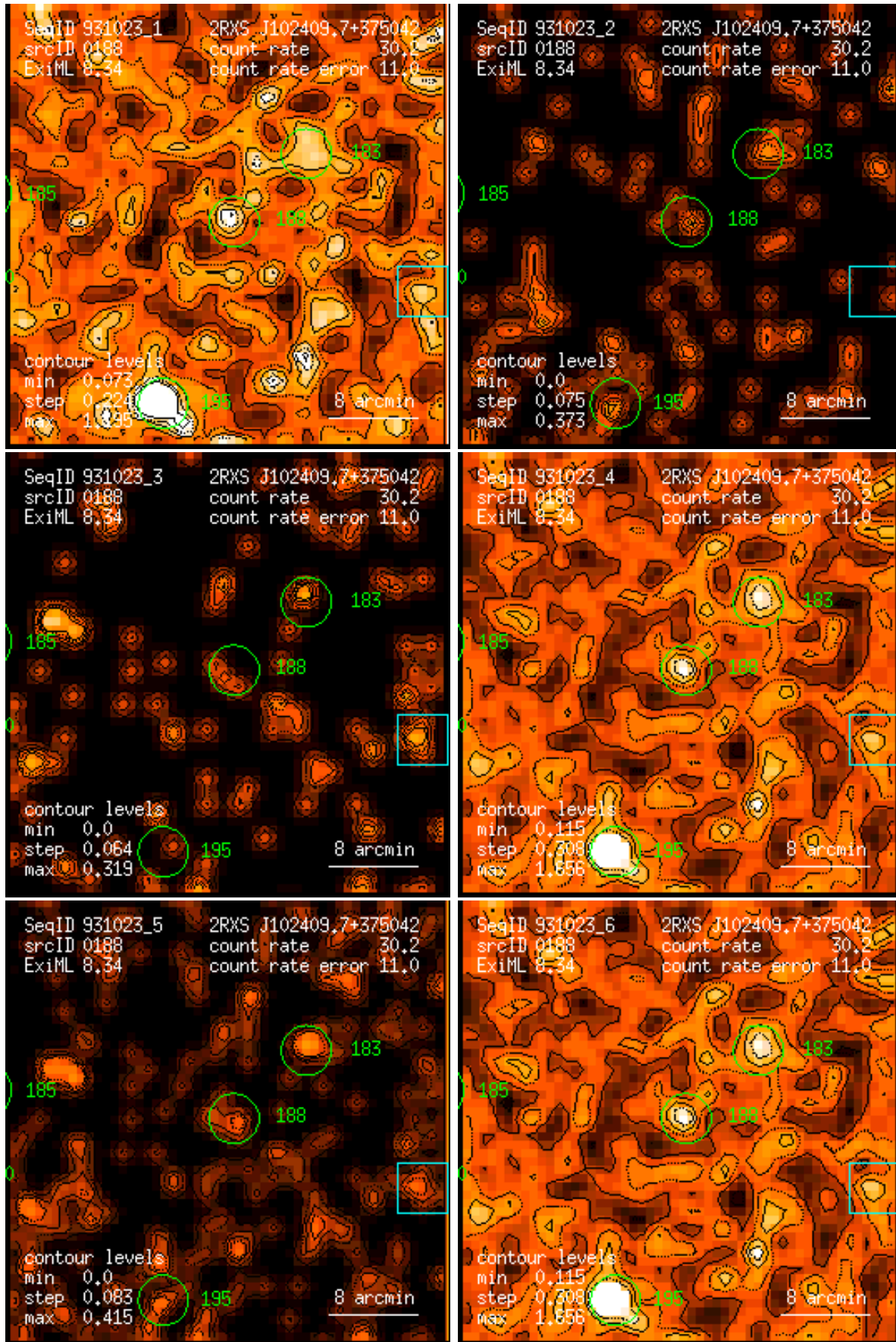
Figure 188: RASS 931023: detection 0188: band rate images, Gaussian filter: (1) PSPC channels 11 – 41, (2) 52 – 90, (3) 91 – 201, (4) 11 – 235, (5) 52 – 201, (6) 11 – 201. Broad band rates in counts/ks. Band rate contour levels in counts/ks/arcmin 2 .
