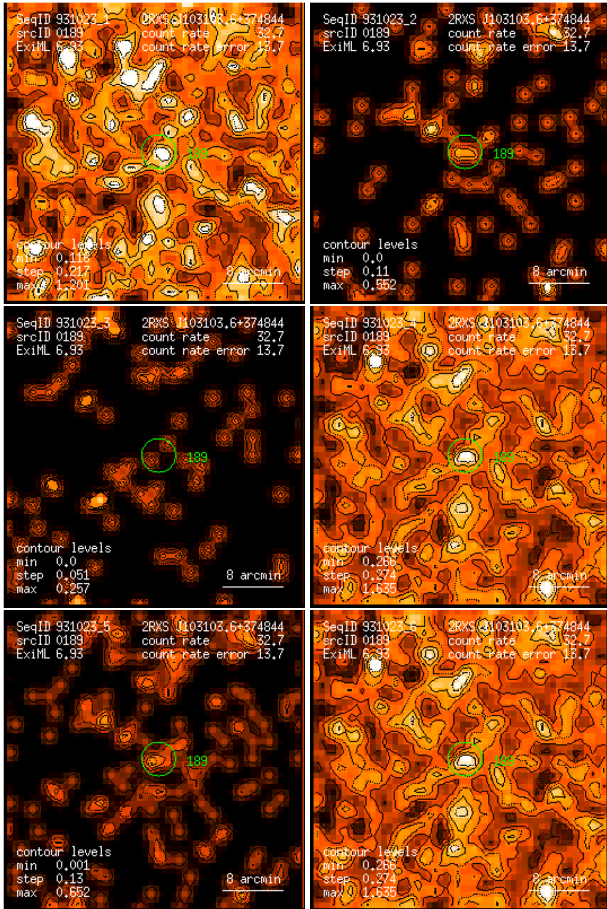
Figure 189: RASS 931023: detection 0189: band rate images, Gaussian filter: (1) PSPC channels 11 – 41, (2) 52 – 90, (3) 91 – 201, (4) 11 – 235, (5) 52 – 201, (6) 11 – 201. Broad band rates in counts/ks. Band rate contour levels in counts/ks/arcmin 2 .
