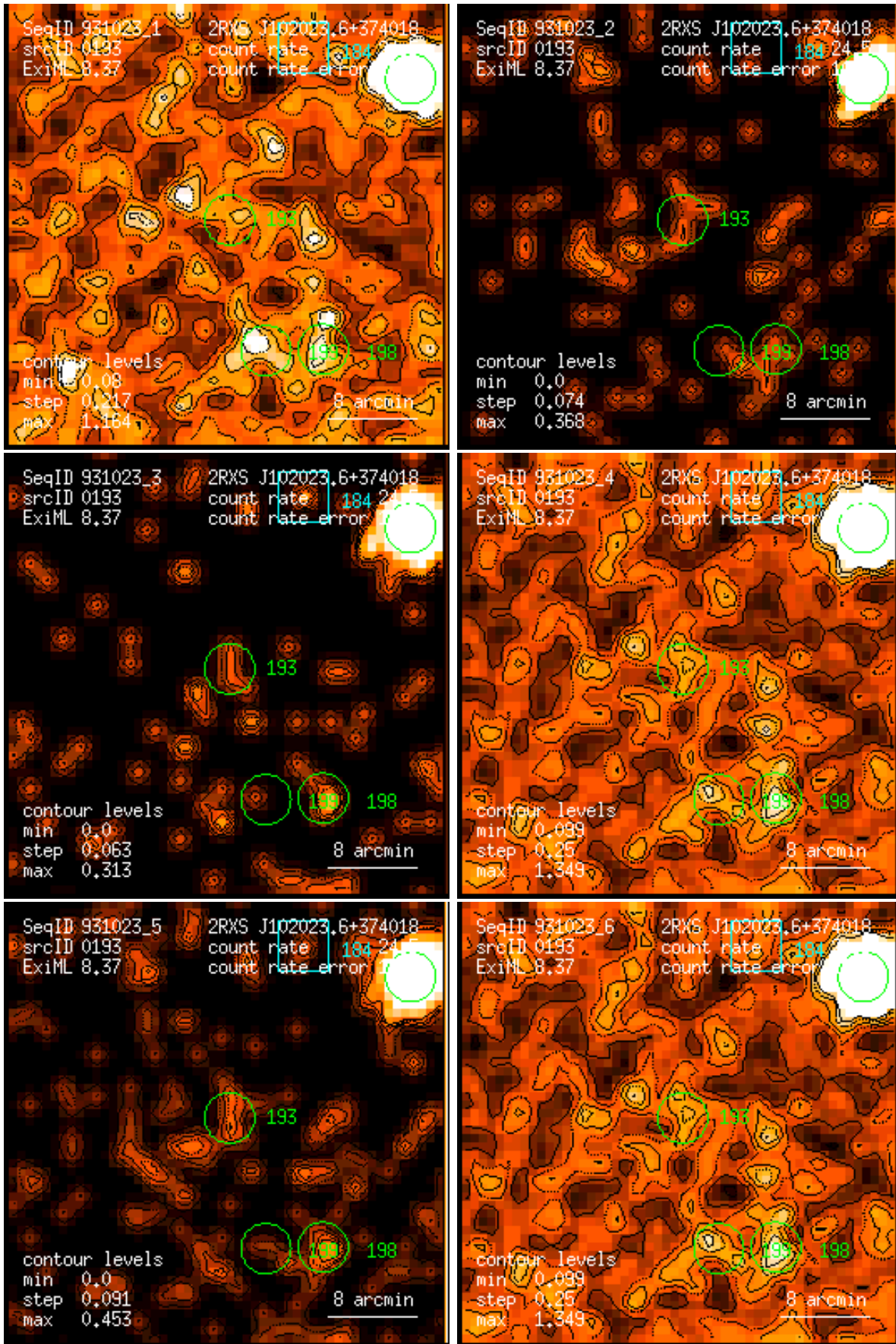
Figure 193: RASS 931023: detection 0193: band rate images, Gaussian filter: (1) PSPC channels 11 – 41, (2) 52 – 90, (3) 91 – 201, (4) 11 – 235, (5) 52 – 201, (6) 11 – 201. Broad band rates in counts/ks. Band rate contour levels in counts/ks/arcmin 2 .
