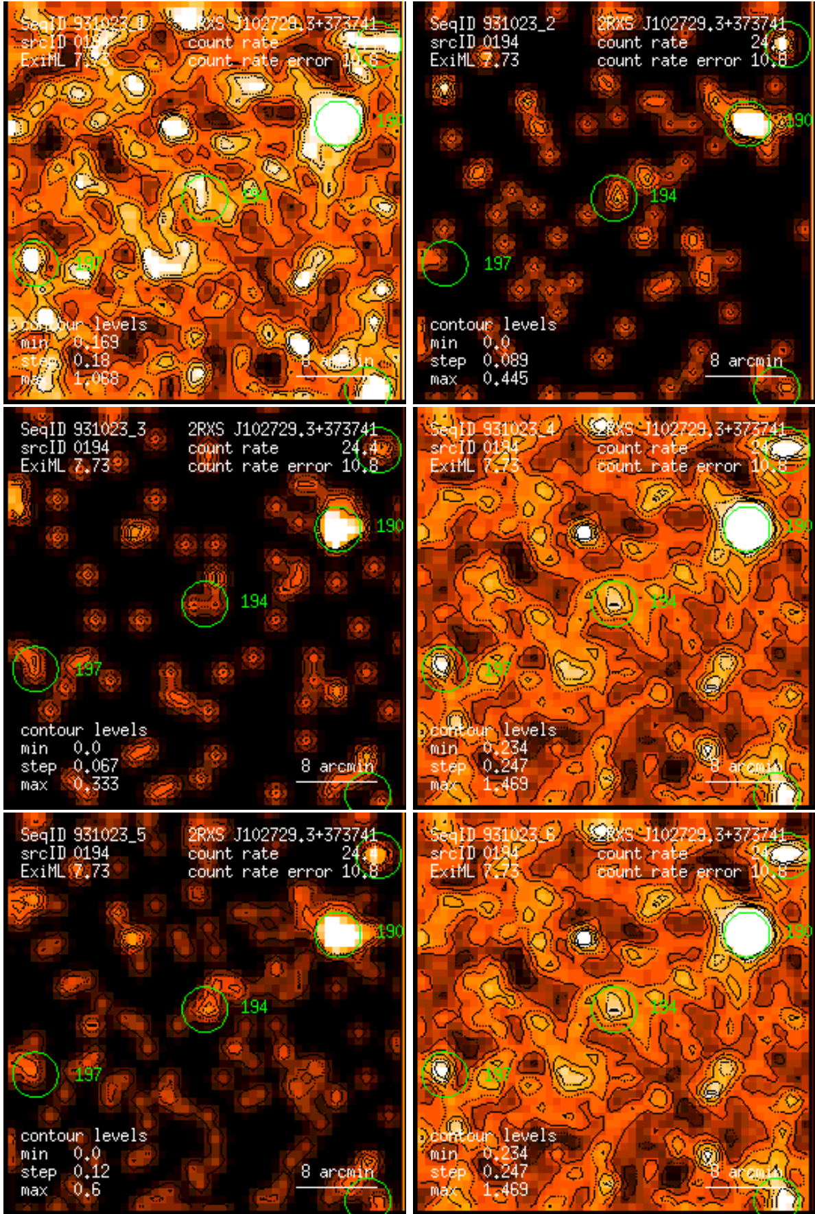
Figure 194: RASS 931023: detection 0194: band rate images, Gaussian filter: (1) PSPC channels 11 – 41, (2) 52 – 90, (3) 91 – 201, (4) 11 – 235, (5) 52 – 201, (6) 11 – 201. Broad band rates in counts/ks. Band rate contour levels in counts/ks/arcmin 2 .
