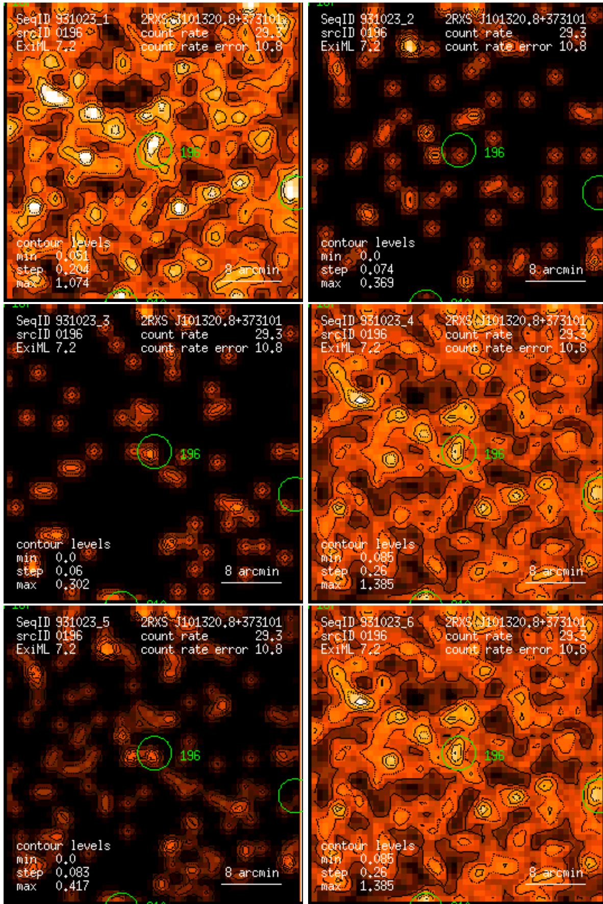
Figure 196: RASS 931023: detection 0196: band rate images, Gaussian filter: (1) PSPC channels 11 – 41, (2) 52 – 90, (3) 91 – 201, (4) 11 – 235, (5) 52 – 201, (6) 11 – 201. Broad band rates in counts/ks. Band rate contour levels in counts/ks/arcmin 2 .
