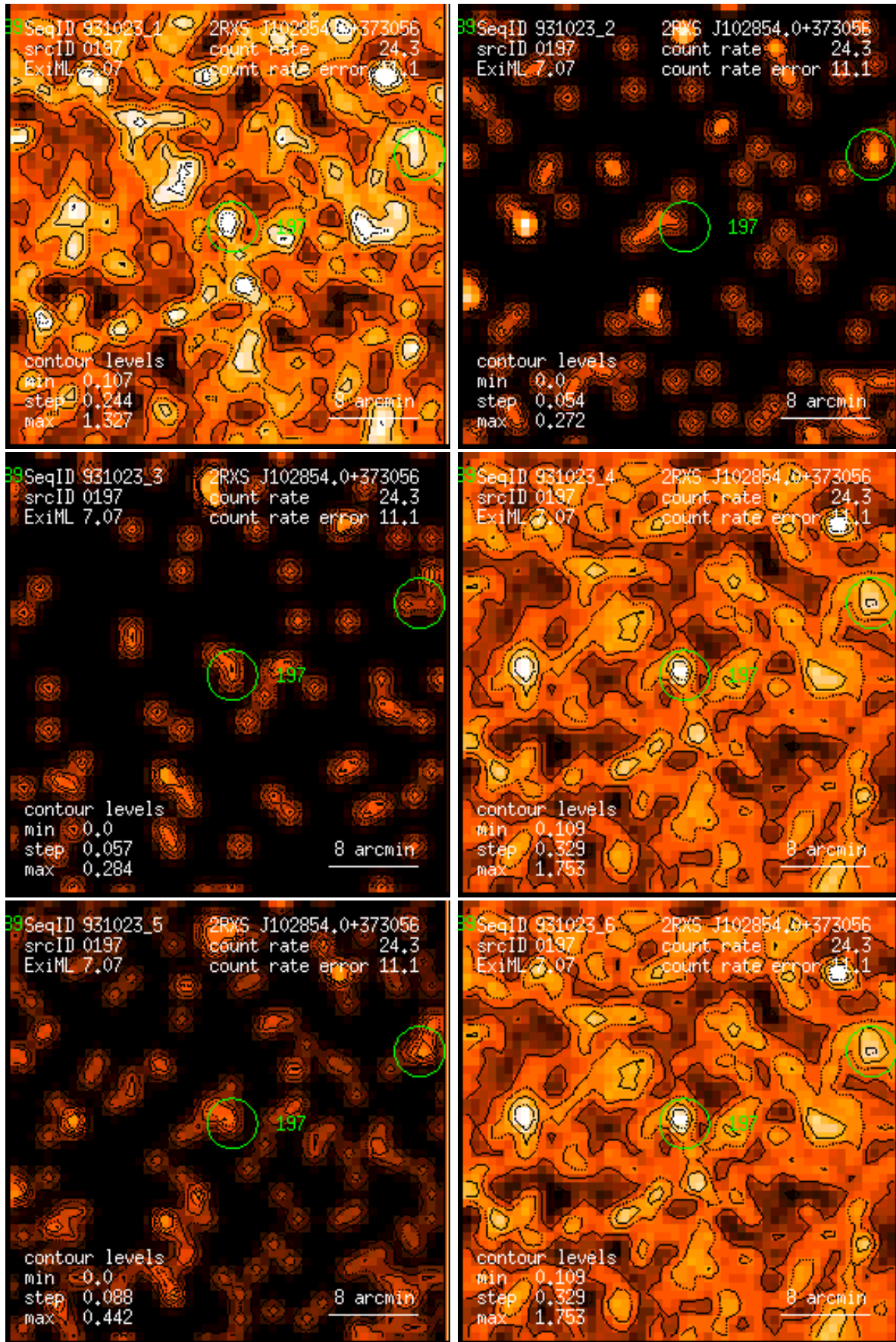
Figure 197: RASS 931023: detection 0197: band rate images, Gaussian filter: (1) PSPC channels 11 – 41, (2) 52 – 90, (3) 91 – 201, (4) 11 – 235, (5) 52 – 201, (6) 11 – 201. Broad band rates in counts/ks. Band rate contour levels in counts/ks/arcmin 2 .
