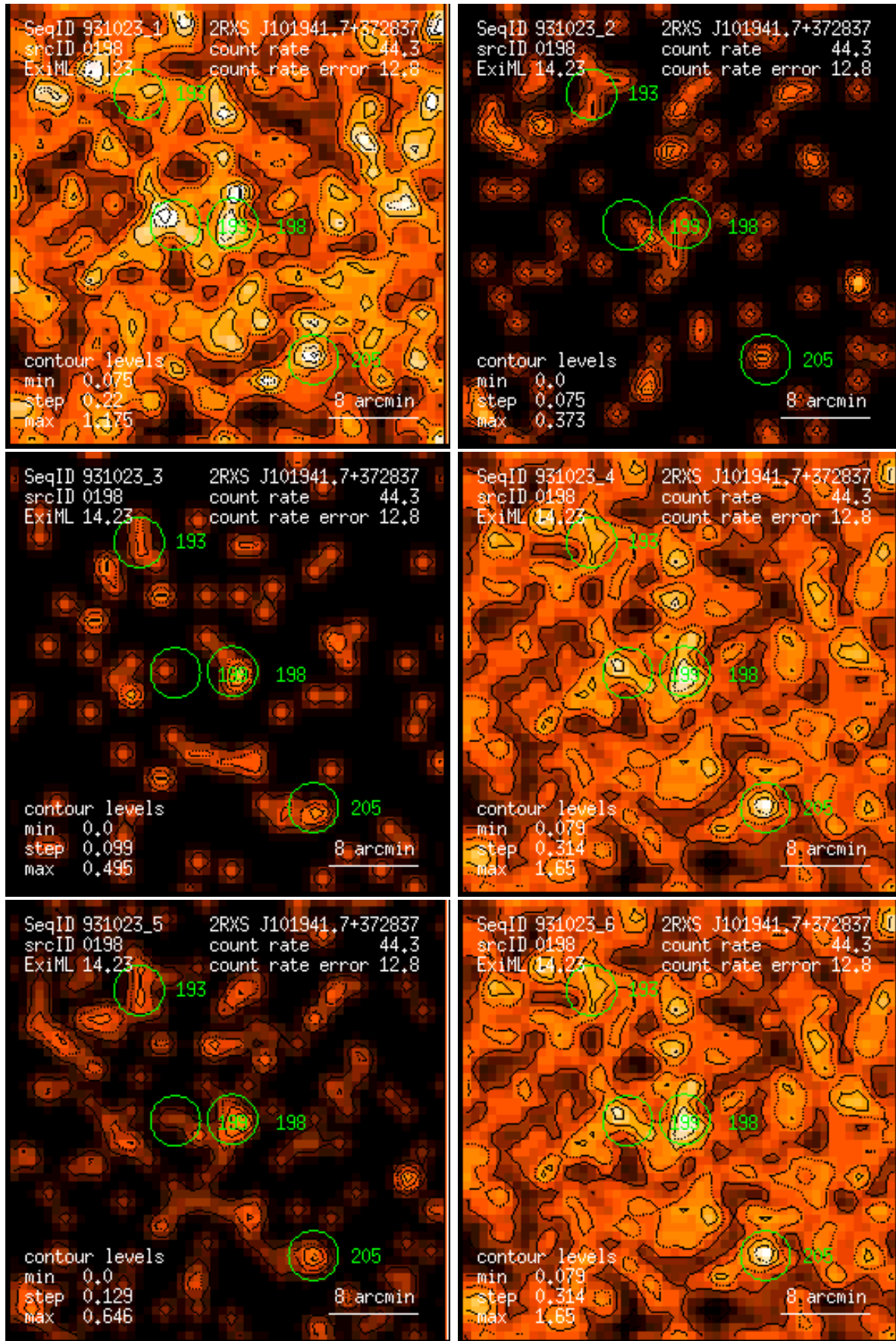
Figure 198: RASS 931023: detection 0198: band rate images, Gaussian filter: (1) PSPC channels 11 – 41, (2) 52 – 90, (3) 91 – 201, (4) 11 – 235, (5) 52 – 201, (6) 11 – 201. Broad band rates in counts/ks. Band rate contour levels in counts/ks/arcmin 2 .
