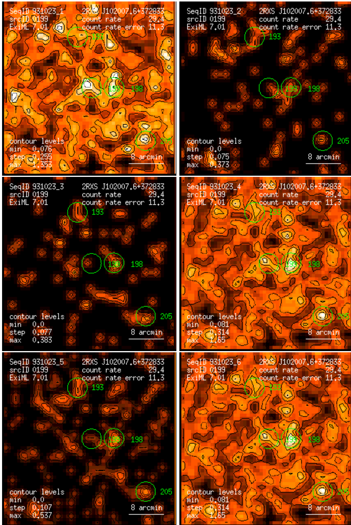
Figure 199: RASS 931023: detection 0199: band rate images, Gaussian filter: (1) PSPC channels 11 – 41, (2) 52 – 90, (3) 91 – 201, (4) 11 – 235, (5) 52 – 201, (6) 11 – 201. Broad band rates in counts/ks. Band rate contour levels in counts/ks/arcmin 2 .
