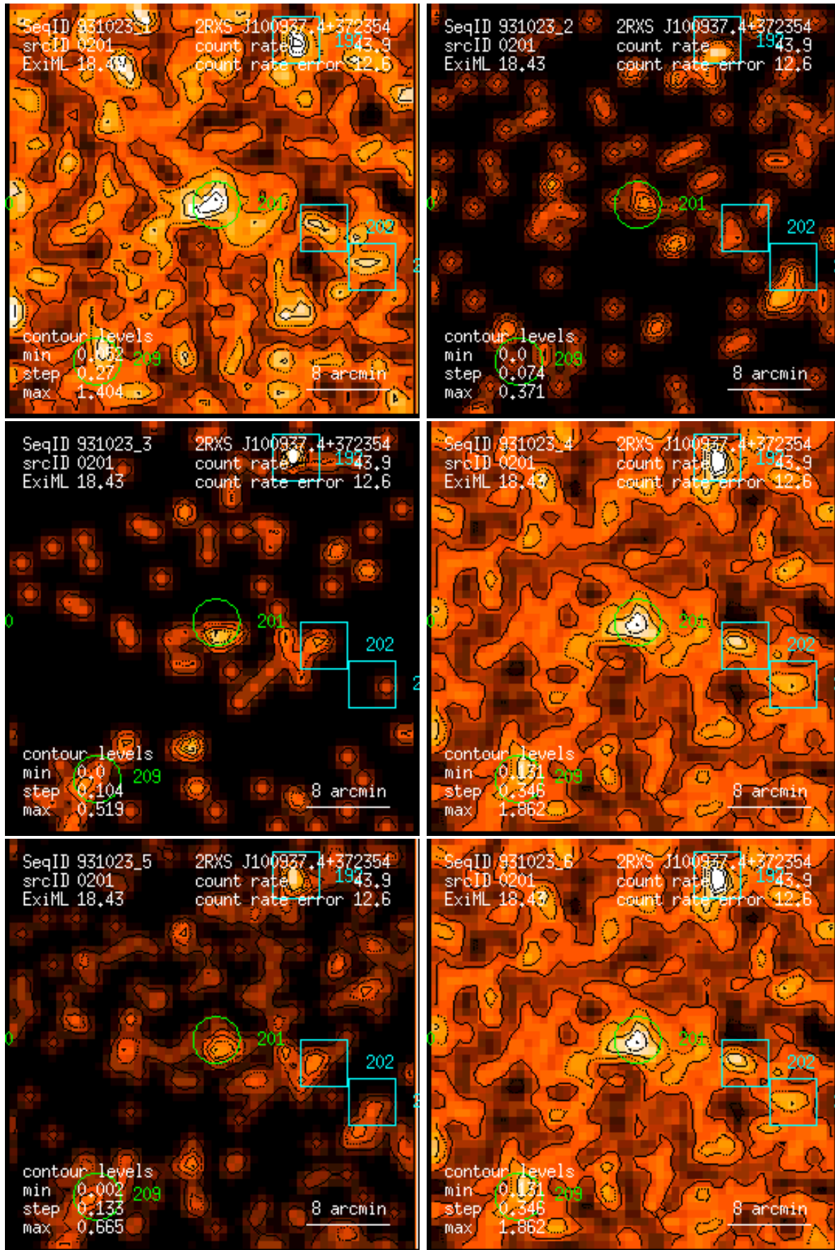
Figure 201: RASS 931023: detection 0201: band rate images, Gaussian filter: (1) PSPC channels 11 – 41, (2) 52 – 90, (3) 91 – 201, (4) 11 – 235, (5) 52 – 201, (6) 11 – 201. Broad band rates in counts/ks. Band rate contour levels in counts/ks/arcmin 2 .
