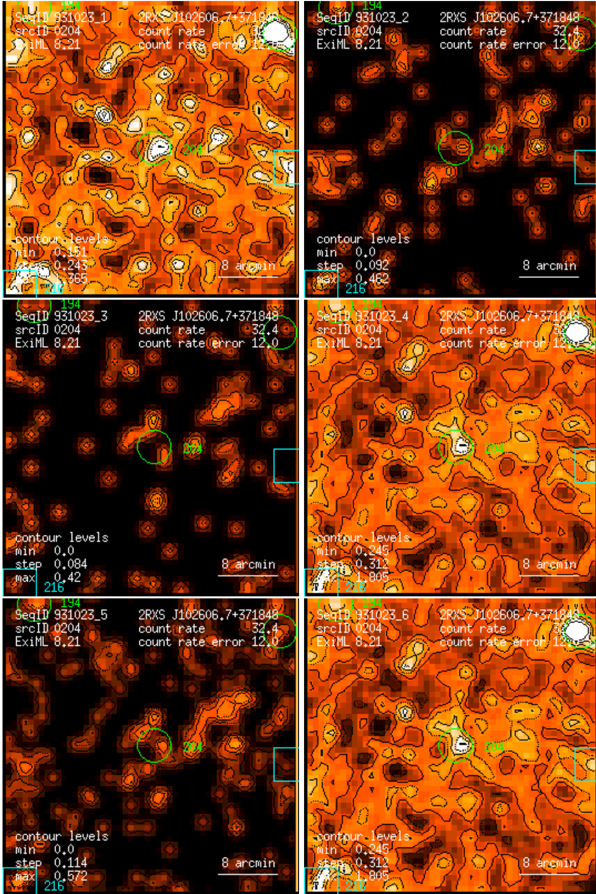
Figure 204: RASS 931023: detection 0204: band rate images, Gaussian filter: (1) PSPC channels 11 – 41, (2) 52 – 90, (3) 91 – 201, (4) 11 – 235, (5) 52 – 201, (6) 11 – 201. Broad band rates in counts/ks. Band rate contour levels in counts/ks/arcmin 2 .
