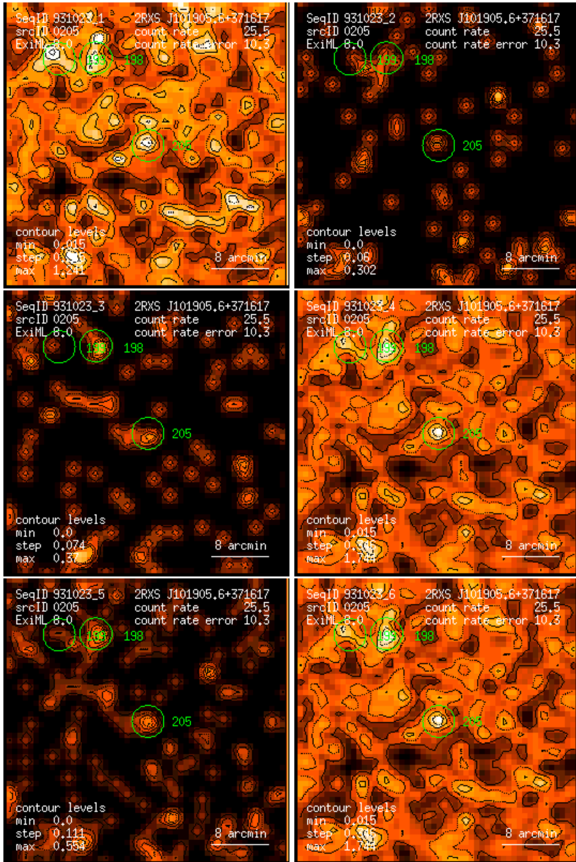
Figure 205: RASS 931023: detection 0205: band rate images, Gaussian filter: (1) PSPC channels 11 – 41, (2) 52 – 90, (3) 91 – 201, (4) 11 – 235, (5) 52 – 201, (6) 11 – 201. Broad band rates in counts/ks. Band rate contour levels in counts/ks/arcmin 2 .
