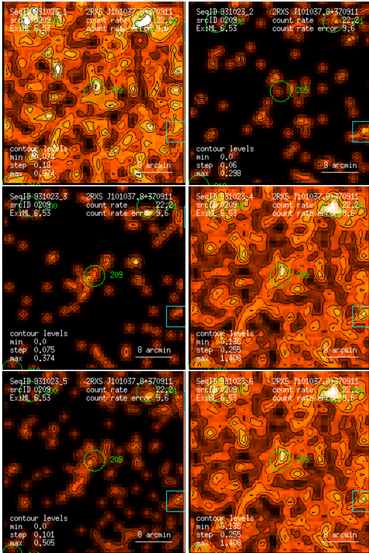
Figure 209: RASS 931023: detection 0209: band rate images, Gaussian filter: (1) PSPC channels 11 – 41, (2) 52 – 90, (3) 91 – 201, (4) 11 – 235, (5) 52 – 201, (6) 11 – 201. Broad band rates in counts/ks. Band rate contour levels in counts/ks/arcmin 2 .
