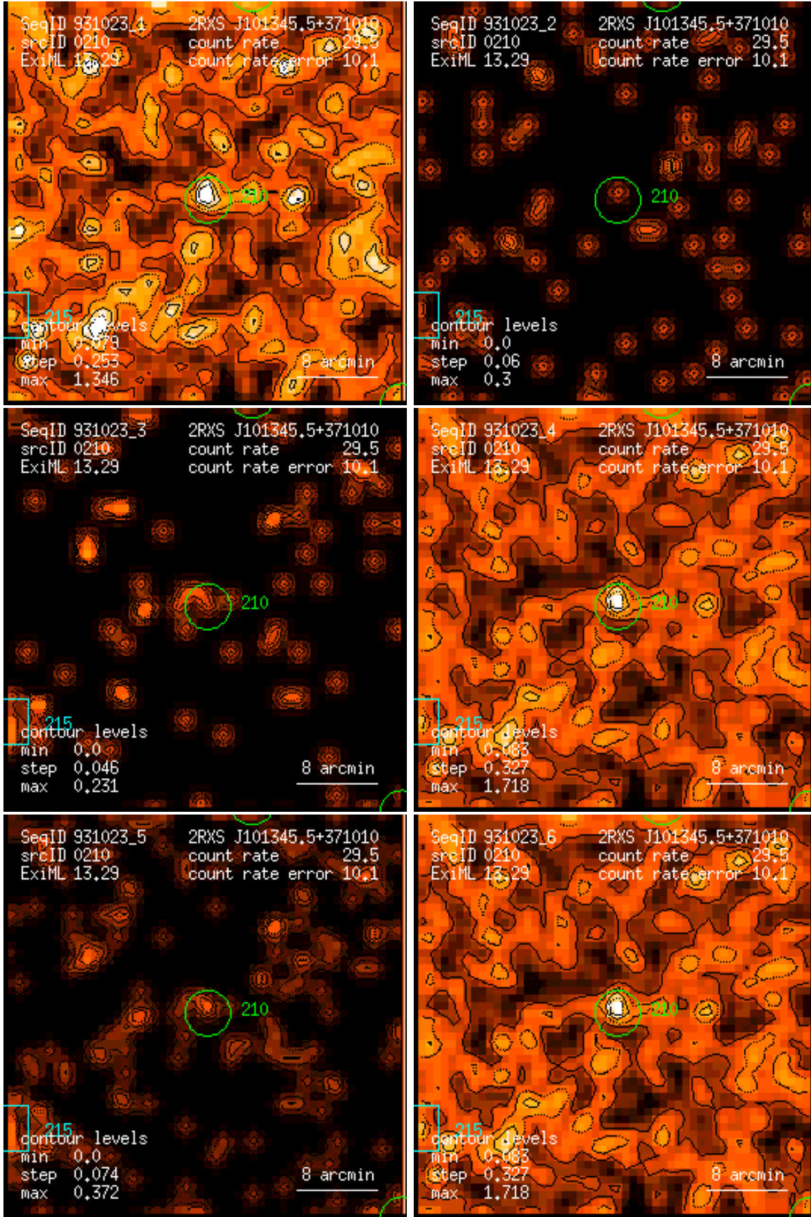
Figure 210: RASS 931023: detection 0210: band rate images, Gaussian filter: (1) PSPC channels 11 – 41, (2) 52 – 90, (3) 91 – 201, (4) 11 – 235, (5) 52 – 201, (6) 11 – 201. Broad band rates in counts/ks. Band rate contour levels in counts/ks/arcmin 2 .
