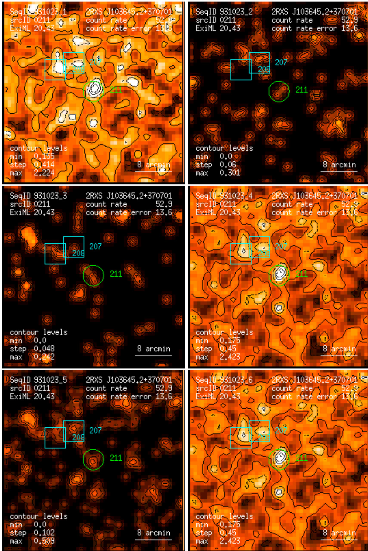
Figure 211: RASS 931023: detection 0211: band rate images, Gaussian filter: (1) PSPC channels 11 – 41, (2) 52 – 90, (3) 91 – 201, (4) 11 – 235, (5) 52 – 201, (6) 11 – 201. Broad band rates in counts/ks. Band rate contour levels in counts/ks/arcmin 2 .
