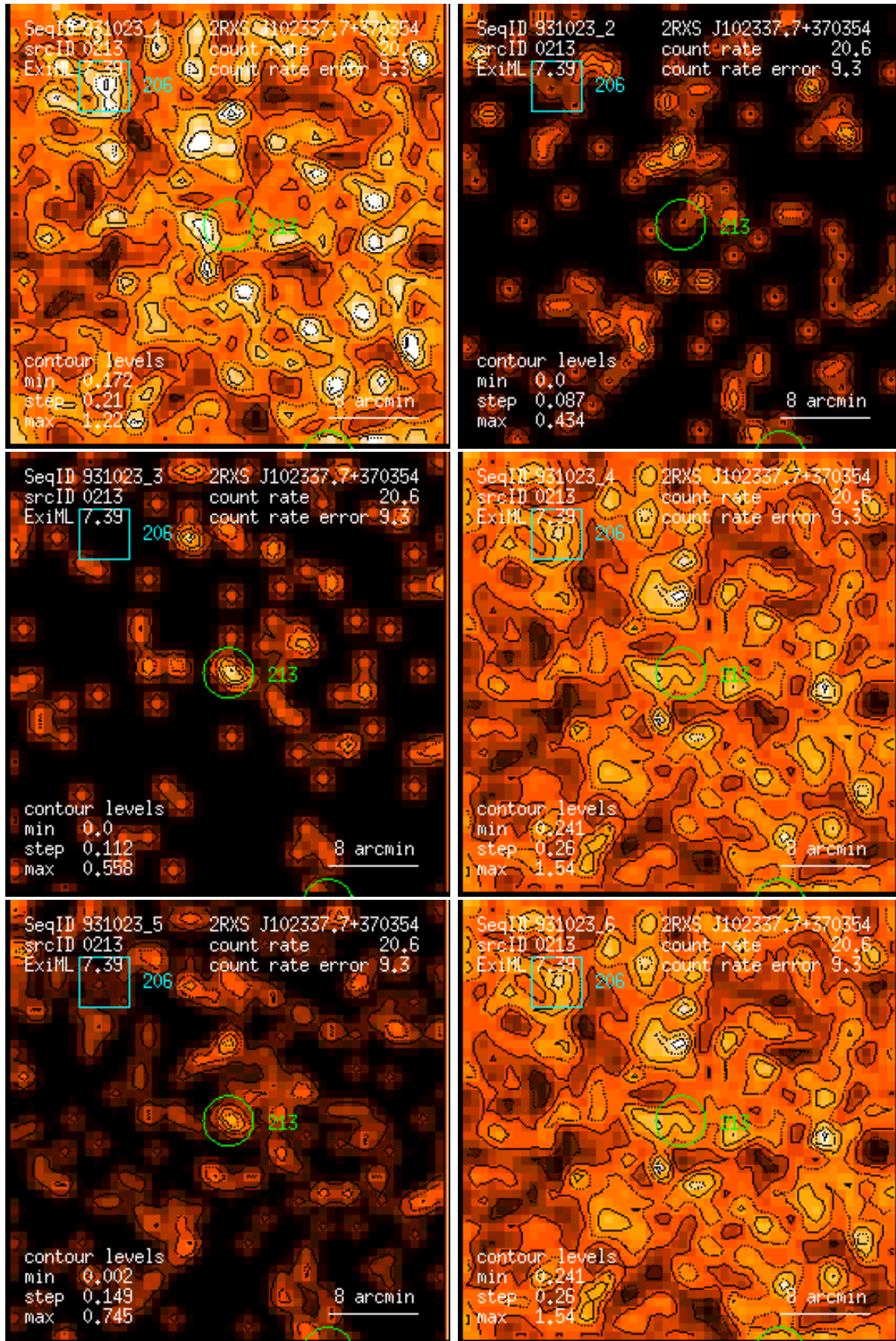
Figure 213: RASS 931023: detection 0213: band rate images, Gaussian filter: (1) PSPC channels 11 – 41, (2) 52 – 90, (3) 91 – 201, (4) 11 – 235, (5) 52 – 201, (6) 11 – 201. Broad band rates in counts/ks. Band rate contour levels in counts/ks/arcmin 2 .
