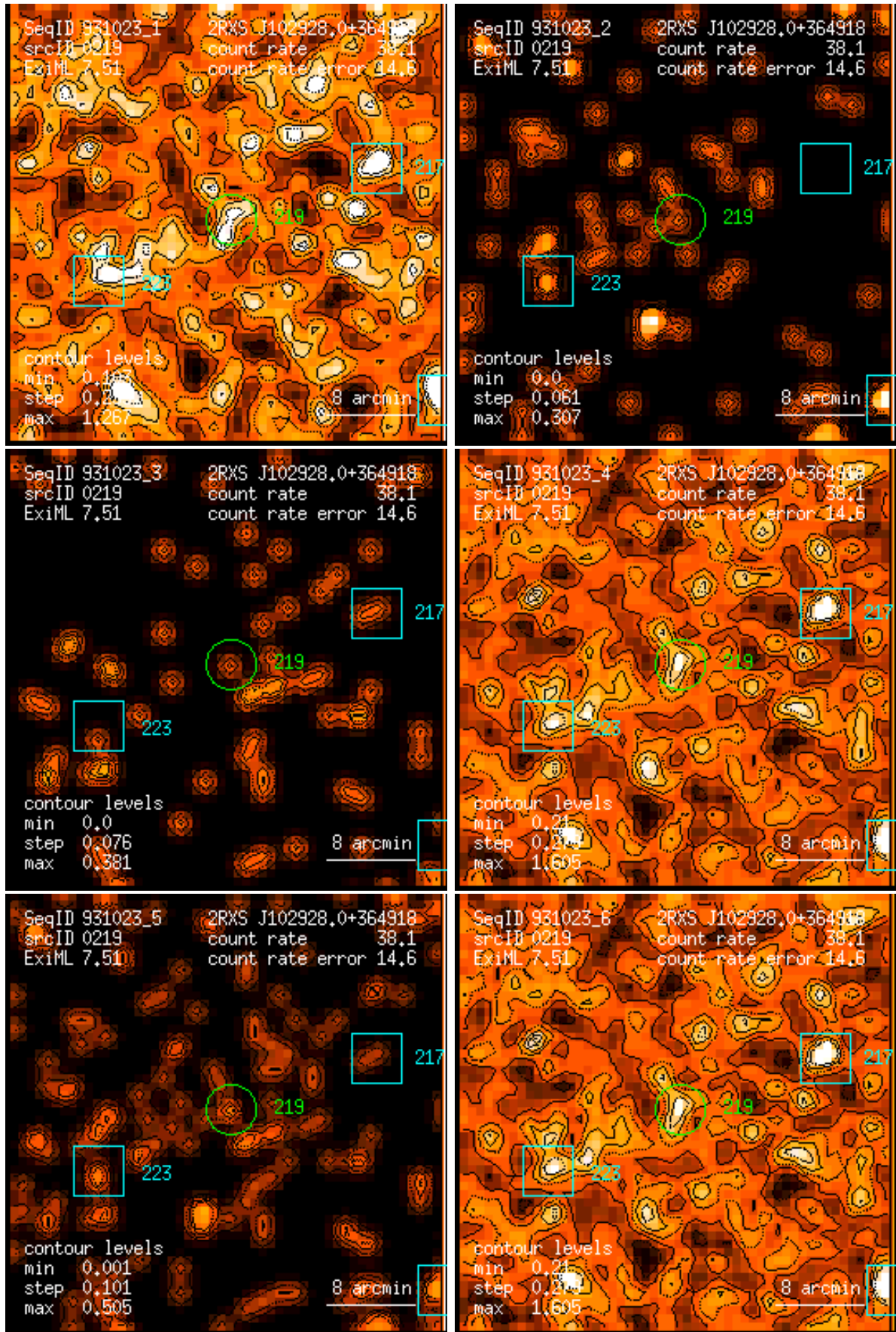
Figure 219: RASS 931023: detection 0219: band rate images, Gaussian filter: (1) PSPC channels 11 – 41, (2) 52 – 90, (3) 91 – 201, (4) 11 – 235, (5) 52 – 201, (6) 11 – 201. Broad band rates in counts/ks. Band rate contour levels in counts/ks/arcmin 2 .
