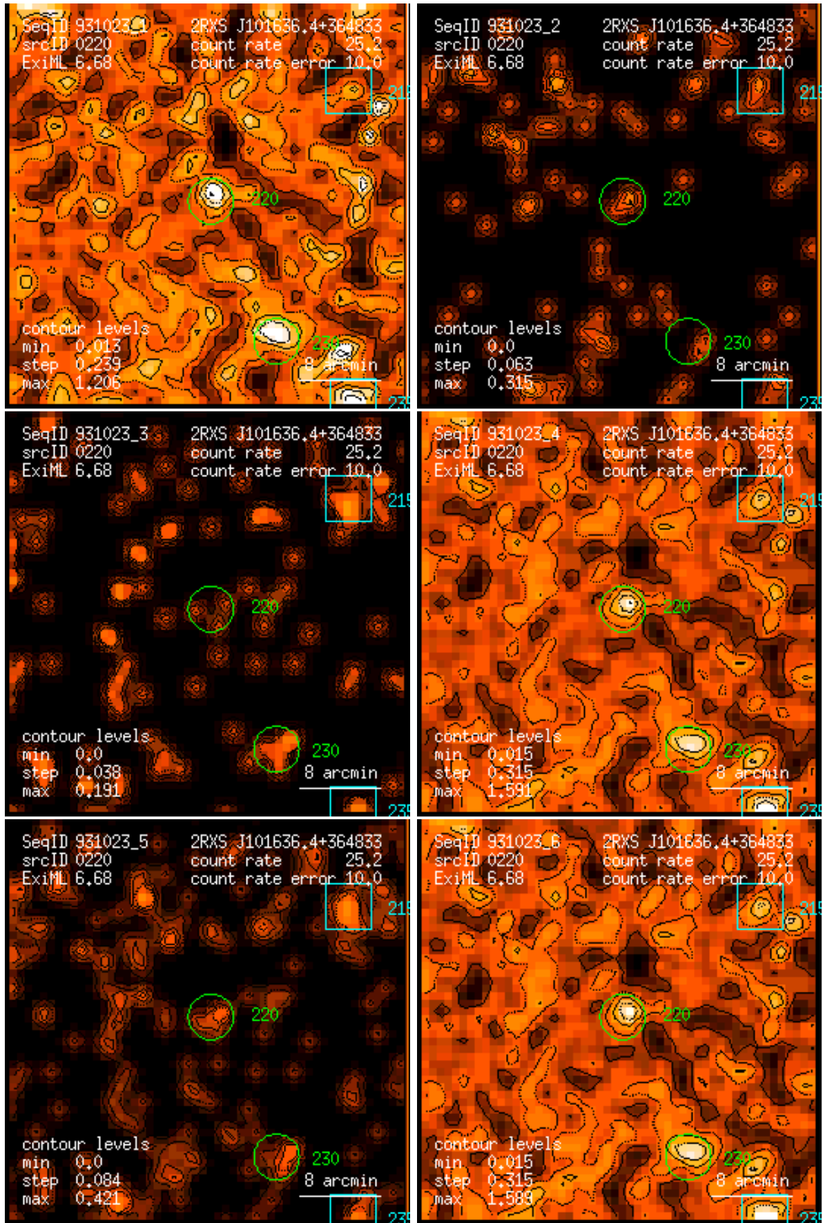
Figure 220: RASS 931023: detection 0220: band rate images, Gaussian filter: (1) PSPC channels 11 – 41, (2) 52 – 90, (3) 91 – 201, (4) 11 – 235, (5) 52 – 201, (6) 11 – 201. Broad band rates in counts/ks. Band rate contour levels in counts/ks/arcmin 2 .
